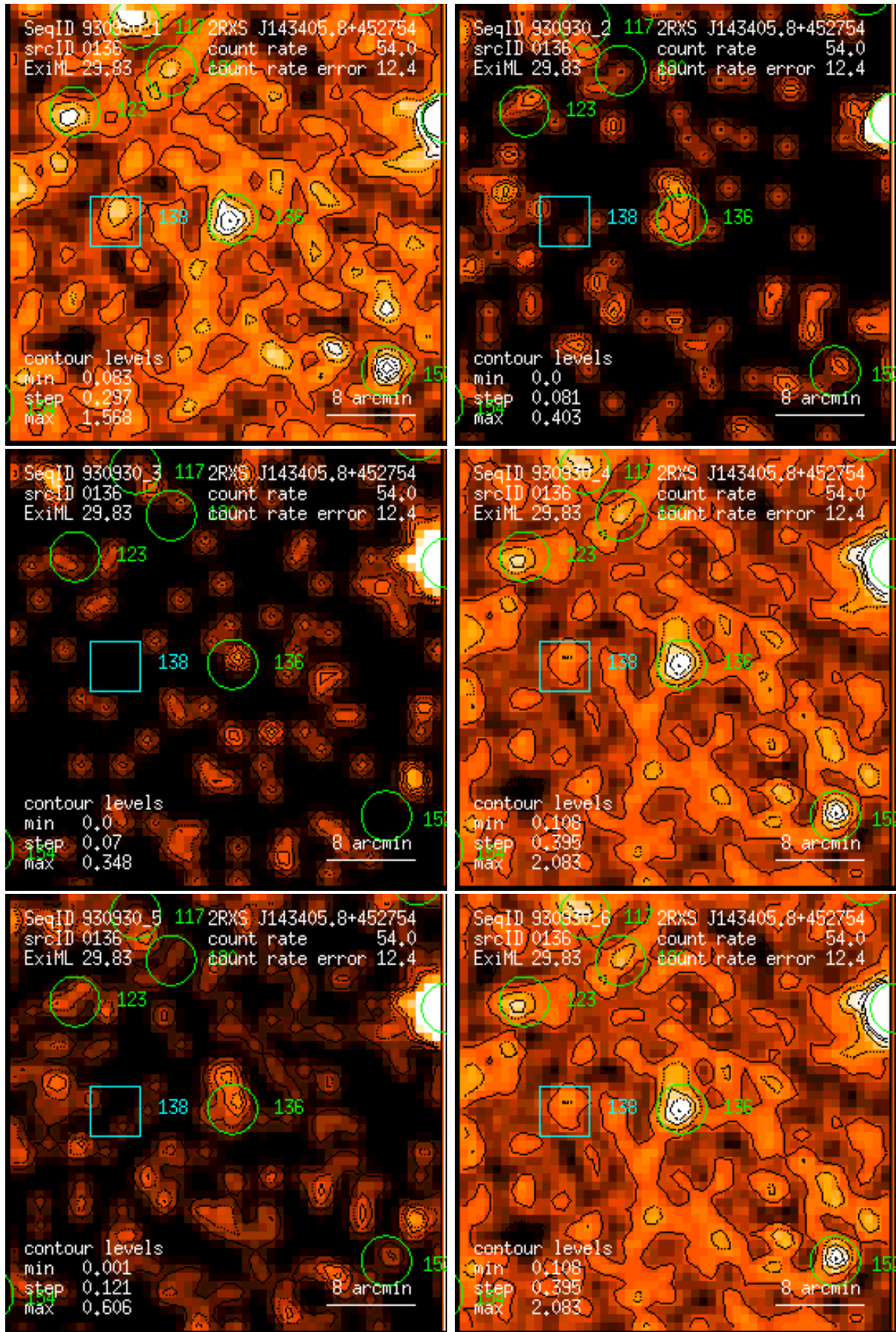
Figure 136: RASS 930930: detection 0136: band rate images, Gaussian filter: (1) PSPC channels 11 – 41, (2) 52 – 90, (3) 91 – 201, (4) 11 – 235, (5) 52 – 201, (6) 11 – 201. Broad band rates in counts/ks. Band rate contour levels in counts/ks/arcmin 2 .
