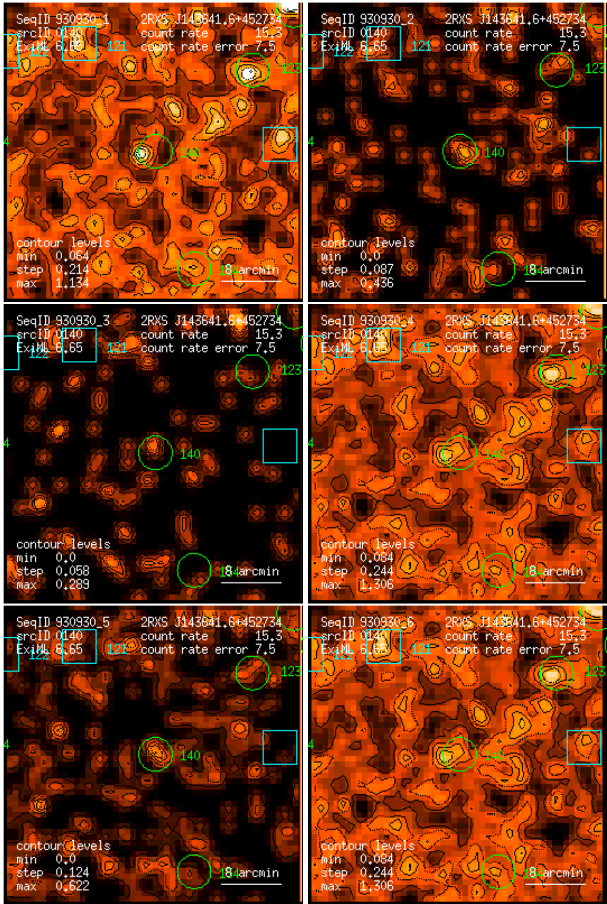
Figure 140: RASS 930930: detection 0140: band rate images, Gaussian filter: (1) PSPC channels 11 – 41, (2) 52 – 90, (3) 91 – 201, (4) 11 – 235, (5) 52 – 201, (6) 11 – 201. Broad band rates in counts/ks. Band rate contour levels in counts/ks/arcmin 2 .
