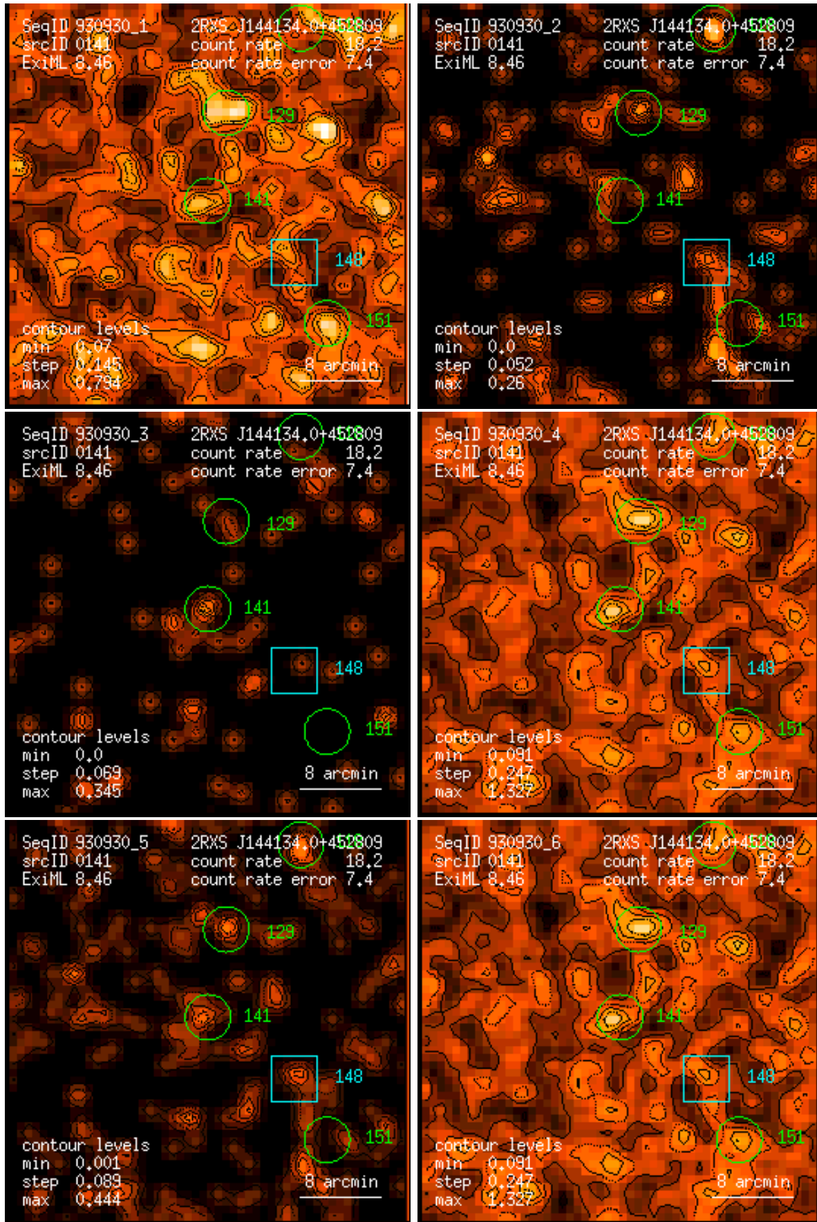
Figure 141: RASS 930930: detection 0141: band rate images, Gaussian filter: (1) PSPC channels 11 – 41, (2) 52 – 90, (3) 91 – 201, (4) 11 – 235, (5) 52 – 201, (6) 11 – 201. Broad band rates in counts/ks. Band rate contour levels in counts/ks/arcmin 2 .
