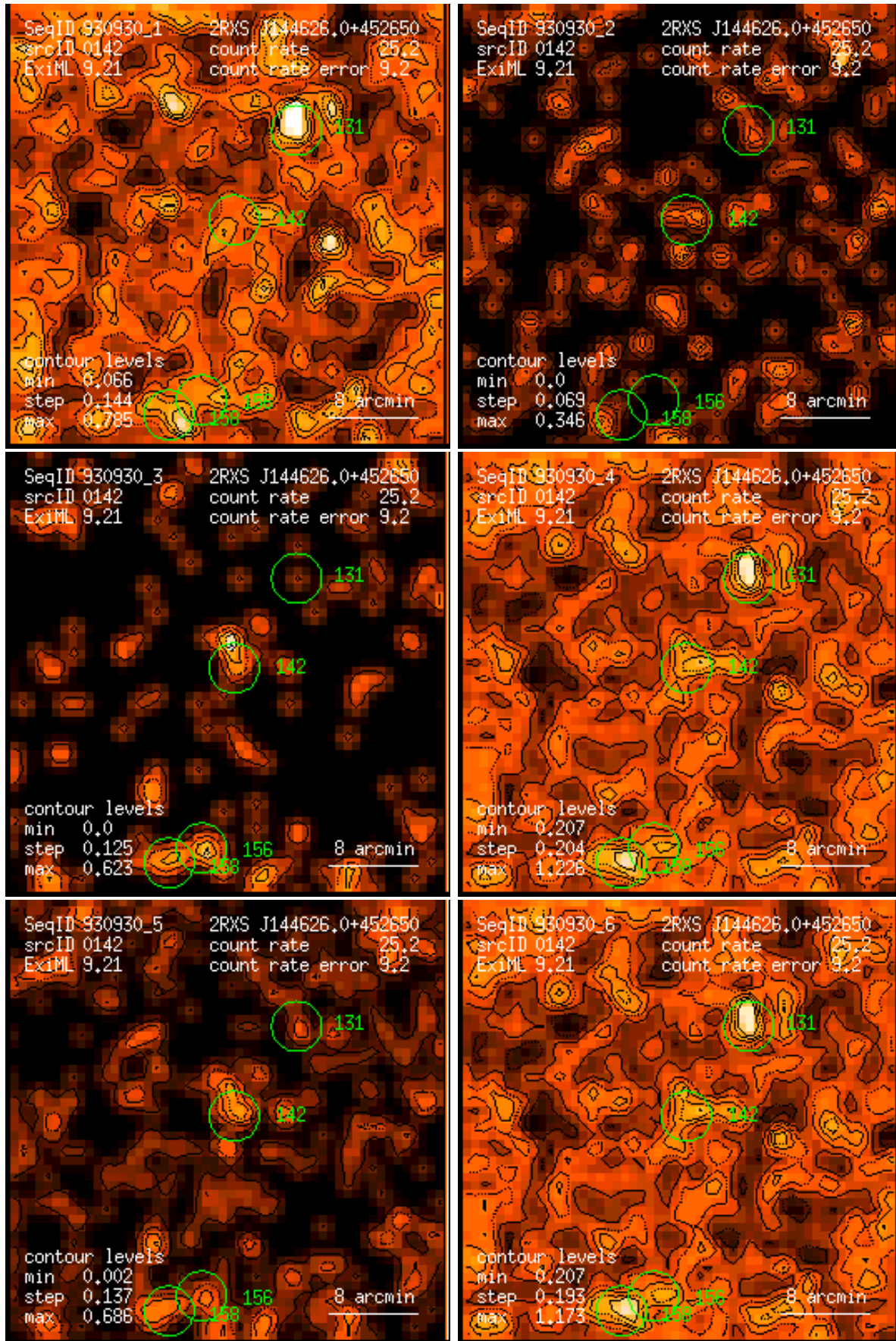
Figure 142: RASS 930930: detection 0142: band rate images, Gaussian filter: (1) PSPC channels 11 – 41, (2) 52 – 90, (3) 91 – 201, (4) 11 – 235, (5) 52 – 201, (6) 11 – 201. Broad band rates in counts/ks. Band rate contour levels in counts/ks/arcmin 2 .
