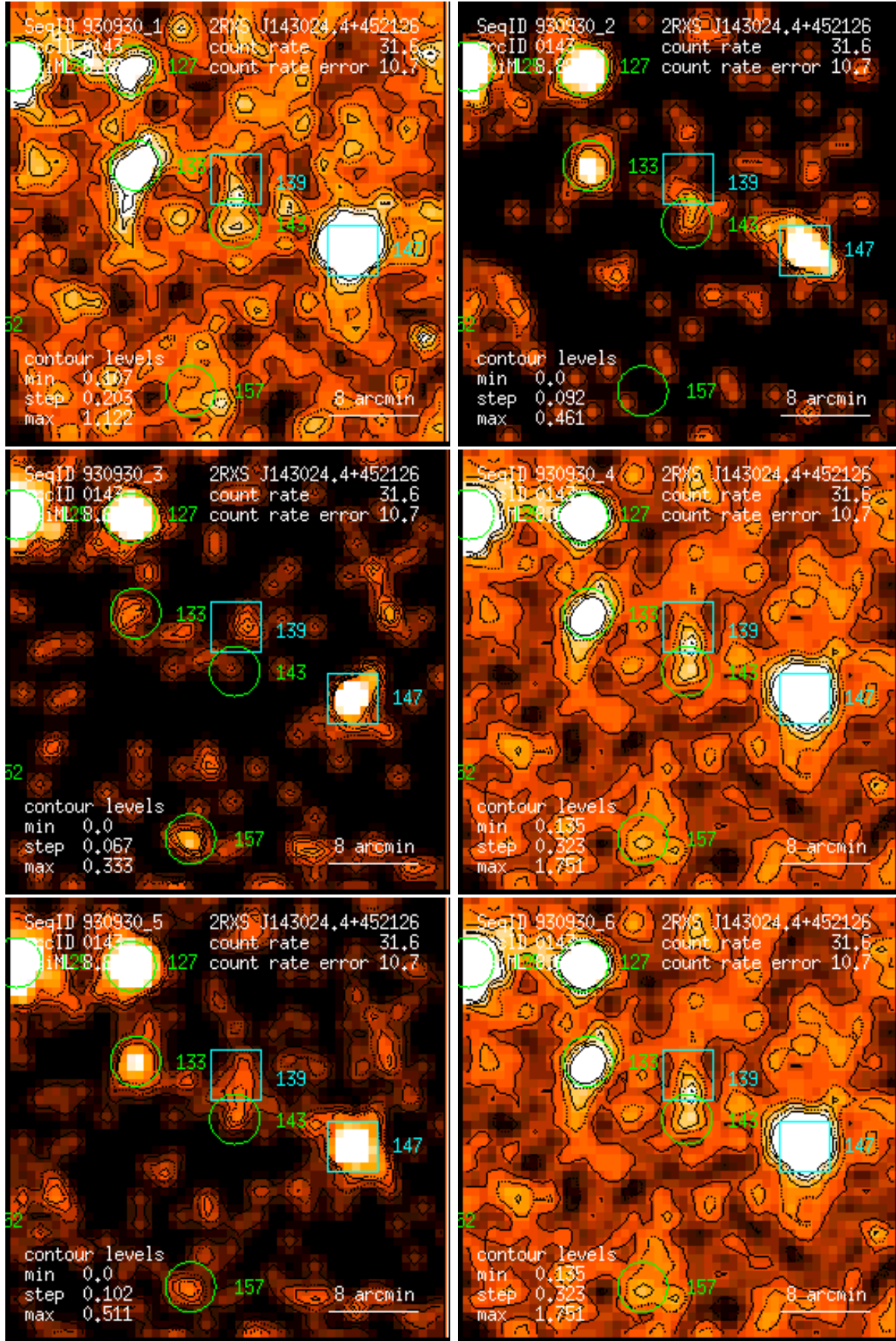
Figure 143: RASS 930930: detection 0143: band rate images, Gaussian filter: (1) PSPC channels 11 – 41, (2) 52 – 90, (3) 91 – 201, (4) 11 – 235, (5) 52 – 201, (6) 11 – 201. Broad band rates in counts/ks. Band rate contour levels in counts/ks/arcmin 2 .
