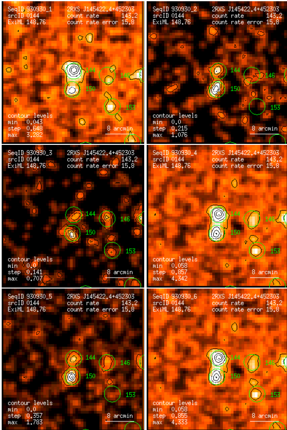
Figure 144: RASS 930930: detection 0144: band rate images, Gaussian filter: (1) PSPC channels 11 – 41, (2) 52 – 90, (3) 91 – 201, (4) 11 – 235, (5) 52 – 201, (6) 11 – 201. Broad band rates in counts/ks. Band rate contour levels in counts/ks/arcmin 2 .
