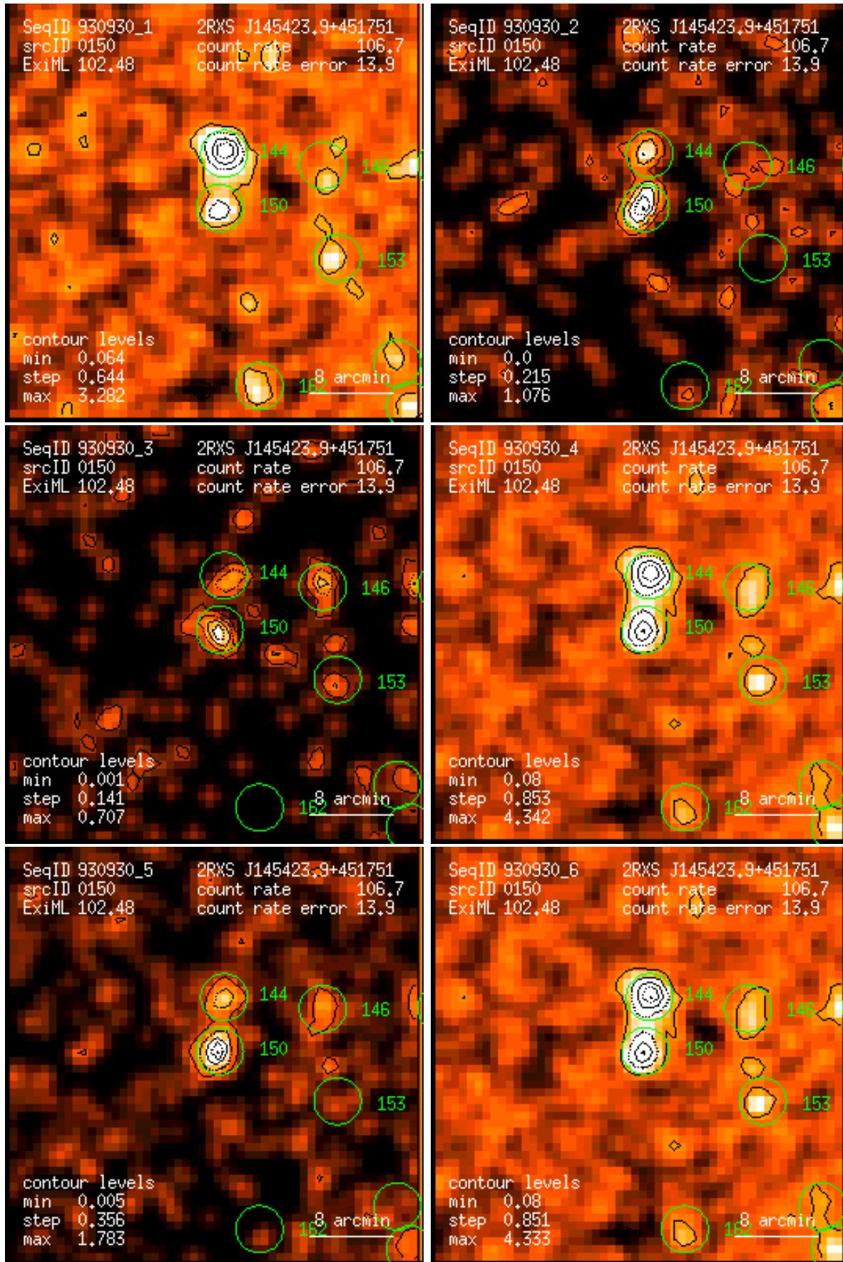
Figure 150: RASS 930930: detection 0150: band rate images, Gaussian filter: (1) PSPC channels 11 – 41, (2) 52 – 90, (3) 91 – 201, (4) 11 – 235, (5) 52 – 201, (6) 11 – 201. Broad band rates in counts/ks. Band rate contour levels in counts/ks/arcmin 2 .
