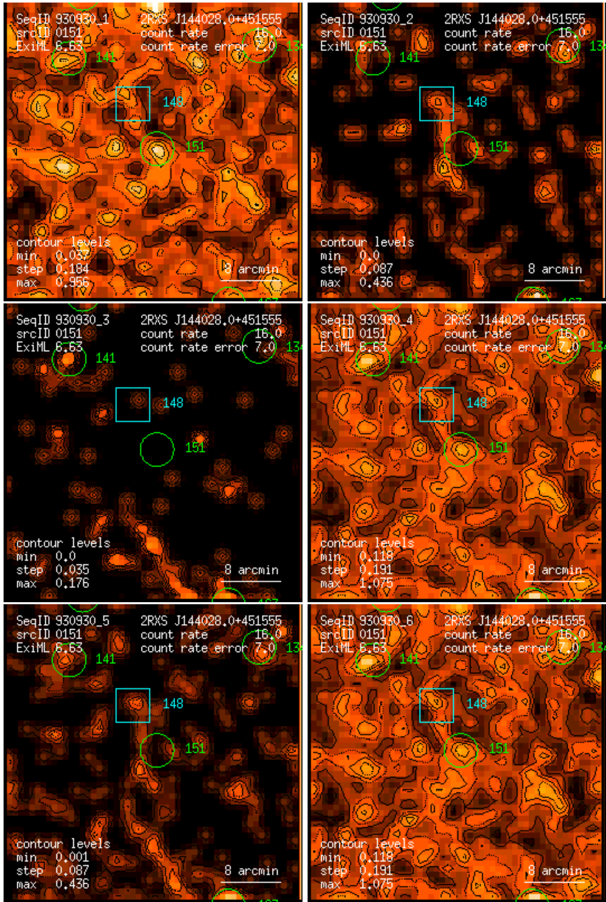
Figure 151: RASS 930930: detection 0151: band rate images, Gaussian filter: (1) PSPC channels 11 – 41, (2) 52 – 90, (3) 91 – 201, (4) 11 – 235, (5) 52 – 201, (6) 11 – 201. Broad band rates in counts/ks. Band rate contour levels in counts/ks/arcmin 2 .
