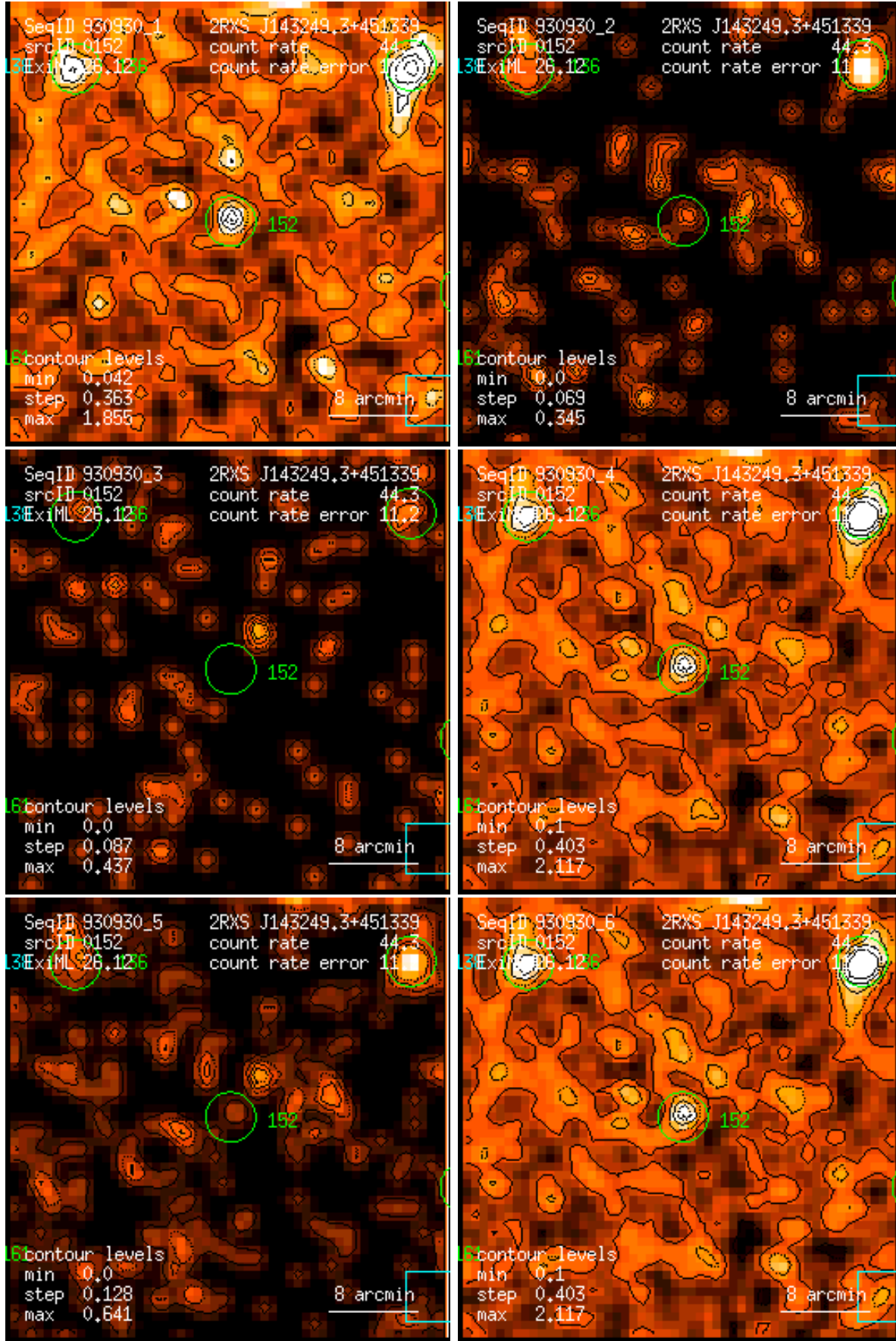
Figure 152: RASS 930930: detection 0152: band rate images, Gaussian filter: (1) PSPC channels 11 – 41, (2) 52 – 90, (3) 91 – 201, (4) 11 – 235, (5) 52 – 201, (6) 11 – 201. Broad band rates in counts/ks. Band rate contour levels in counts/ks/arcmin 2 .
