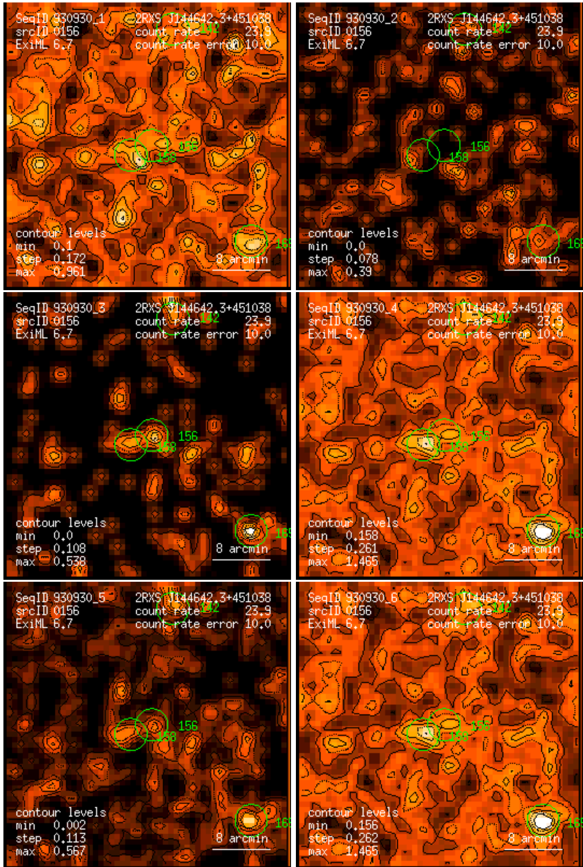
Figure 156: RASS 930930: detection 0156: band rate images, Gaussian filter: (1) PSPC channels 11 – 41, (2) 52 – 90, (3) 91 – 201, (4) 11 – 235, (5) 52 – 201, (6) 11 – 201. Broad band rates in counts/ks. Band rate contour levels in counts/ks/arcmin 2 .
