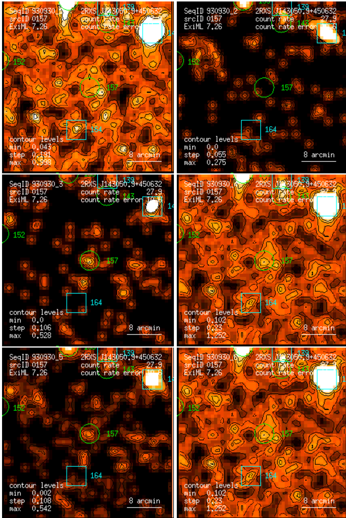
Figure 157: RASS 930930: detection 0157: band rate images, Gaussian filter: (1) PSPC channels 11 – 41, (2) 52 – 90, (3) 91 – 201, (4) 11 – 235, (5) 52 – 201, (6) 11 – 201. Broad band rates in counts/ks. Band rate contour levels in counts/ks/arcmin 2 .
