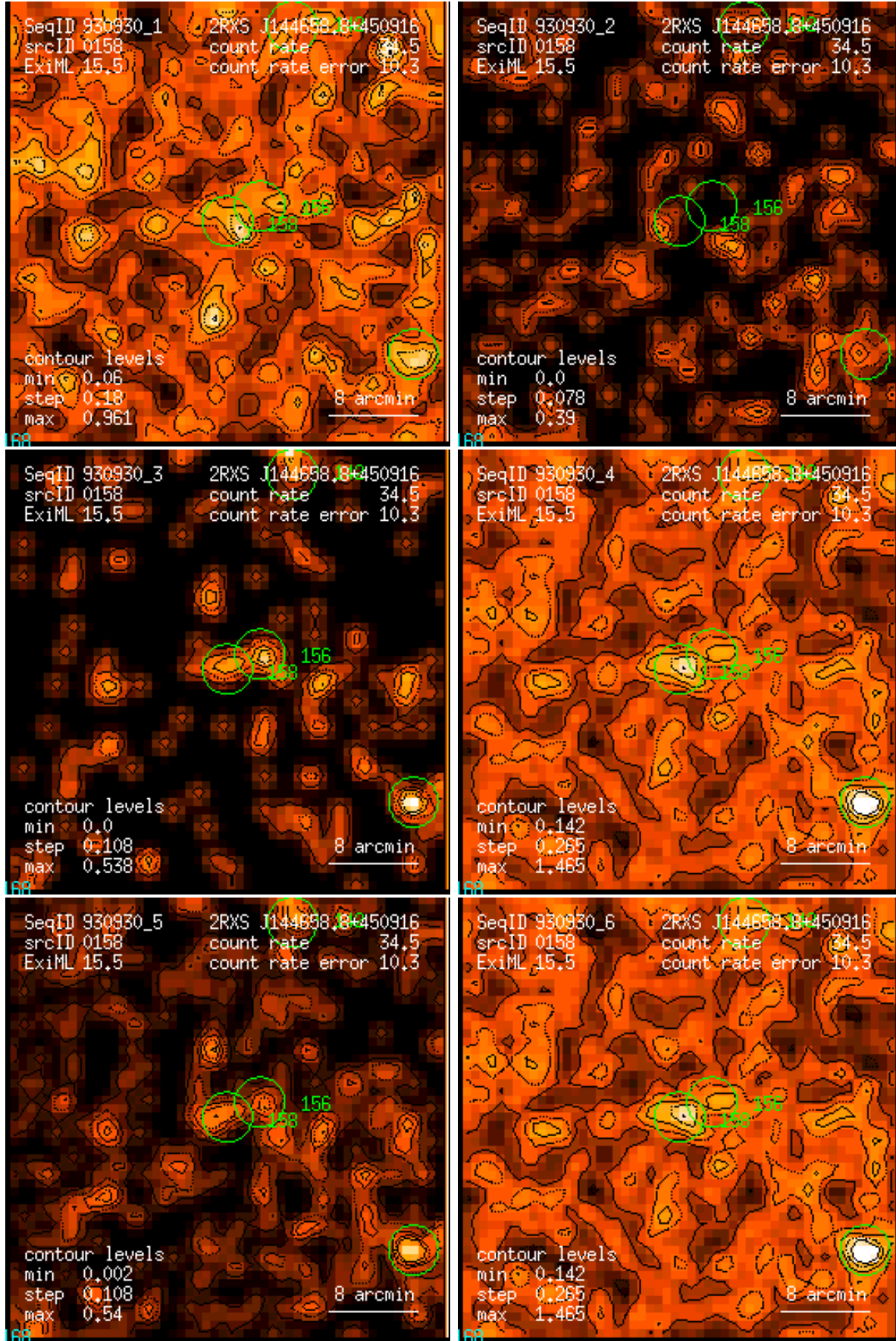
Figure 158: RASS 930930: detection 0158: band rate images, Gaussian filter: (1) PSPC channels 11 – 41, (2) 52 – 90, (3) 91 – 201, (4) 11 – 235, (5) 52 – 201, (6) 11 – 201. Broad band rates in counts/ks. Band rate contour levels in counts/ks/arcmin 2 .
