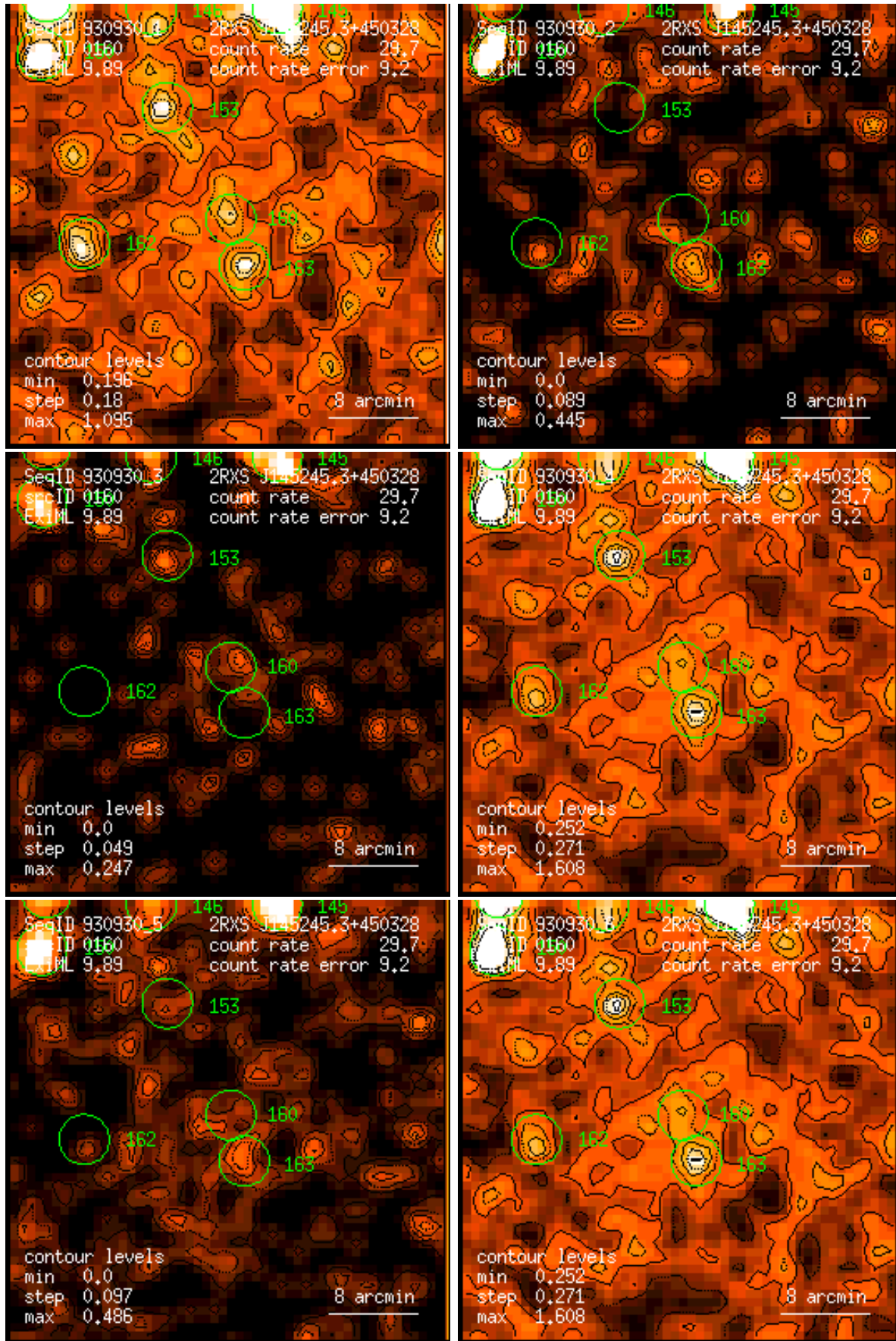
Figure 160: RASS 930930: detection 0160: band rate images, Gaussian filter: (1) PSPC channels 11 – 41, (2) 52 – 90, (3) 91 – 201, (4) 11 – 235, (5) 52 – 201, (6) 11 – 201. Broad band rates in counts/ks. Band rate contour levels in counts/ks/arcmin 2 .
