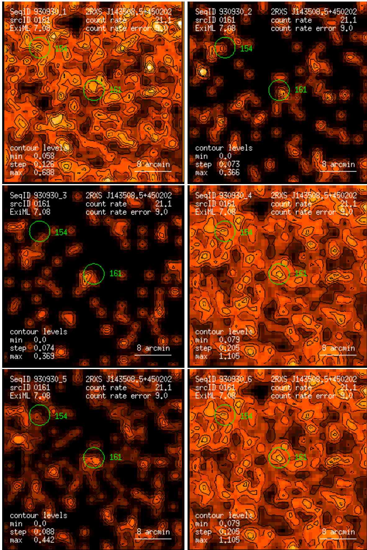
Figure 161: RASS 930930: detection 0161: band rate images, Gaussian filter: (1) PSPC channels 11 – 41, (2) 52 – 90, (3) 91 – 201, (4) 11 – 235, (5) 52 – 201, (6) 11 – 201. Broad band rates in counts/ks. Band rate contour levels in counts/ks/arcmin 2 .
