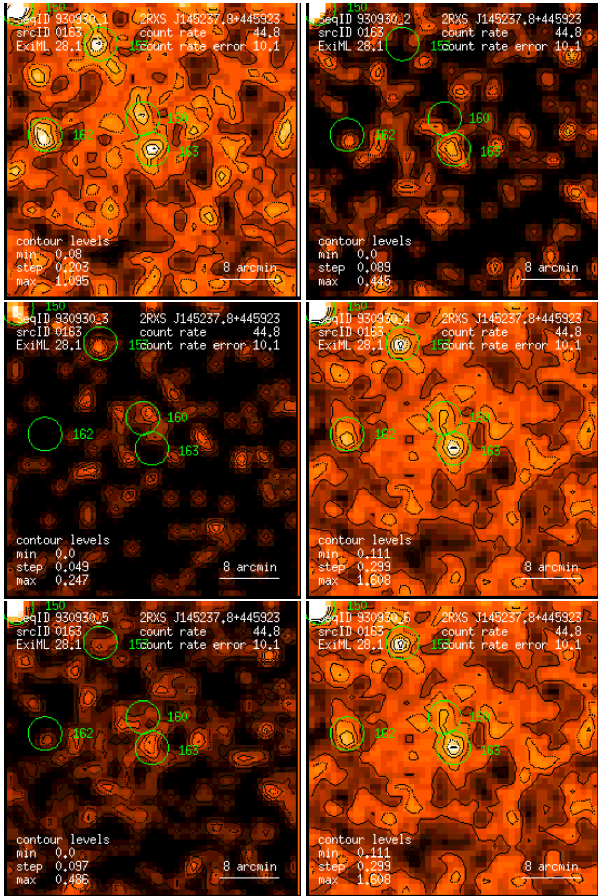
Figure 163: RASS 930930: detection 0163: band rate images, Gaussian filter: (1) PSPC channels 11 – 41, (2) 52 – 90, (3) 91 – 201, (4) 11 – 235, (5) 52 – 201, (6) 11 – 201. Broad band rates in counts/ks. Band rate contour levels in counts/ks/arcmin 2 .
