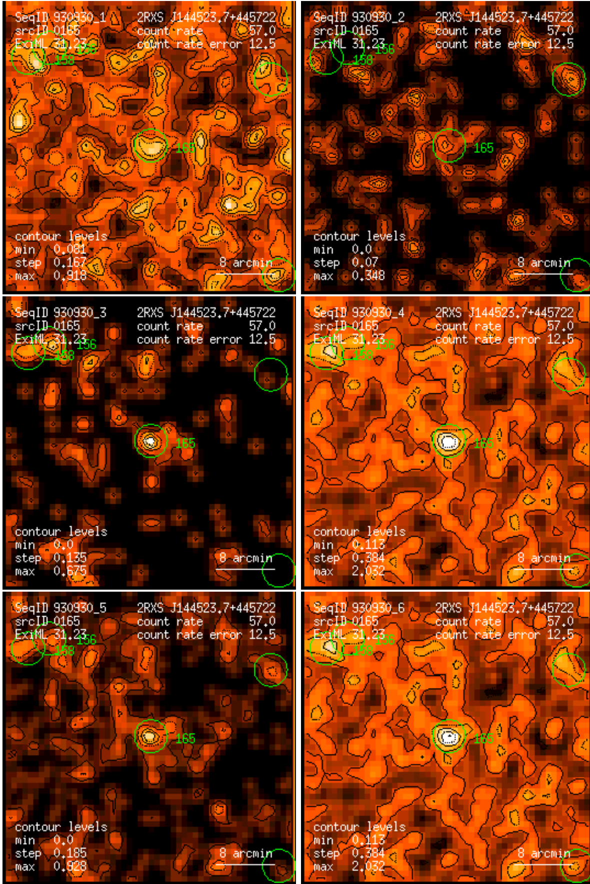
Figure 165: RASS 930930: detection 0165: band rate images, Gaussian filter: (1) PSPC channels 11 – 41, (2) 52 – 90, (3) 91 – 201, (4) 11 – 235, (5) 52 – 201, (6) 11 – 201. Broad band rates in counts/ks. Band rate contour levels in counts/ks/arcmin 2 .
