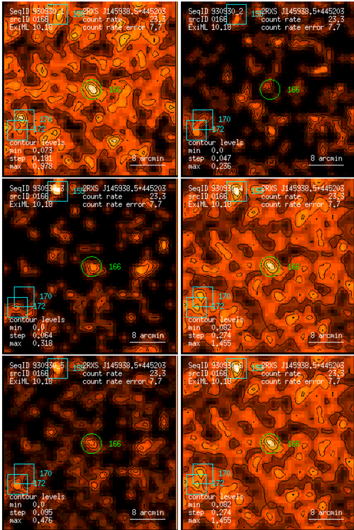
Figure 166: RASS 930930: detection 0166: band rate images, Gaussian filter: (1) PSPC channels 11 – 41, (2) 52 – 90, (3) 91 – 201, (4) 11 – 235, (5) 52 – 201, (6) 11 – 201. Broad band rates in counts/ks. Band rate contour levels in counts/ks/arcmin 2 .
