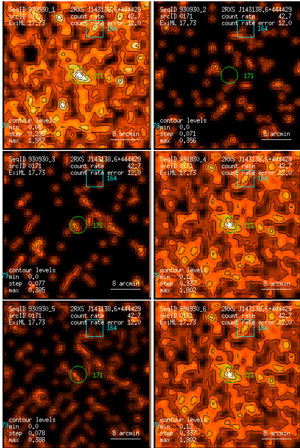
Figure 171: RASS 930930: detection 0171: band rate images, Gaussian filter: (1) PSPC channels 11 – 41, (2) 52 – 90, (3) 91 – 201, (4) 11 – 235, (5) 52 – 201, (6) 11 – 201. Broad band rates in counts/ks. Band rate contour levels in counts/ks/arcmin 2 .
