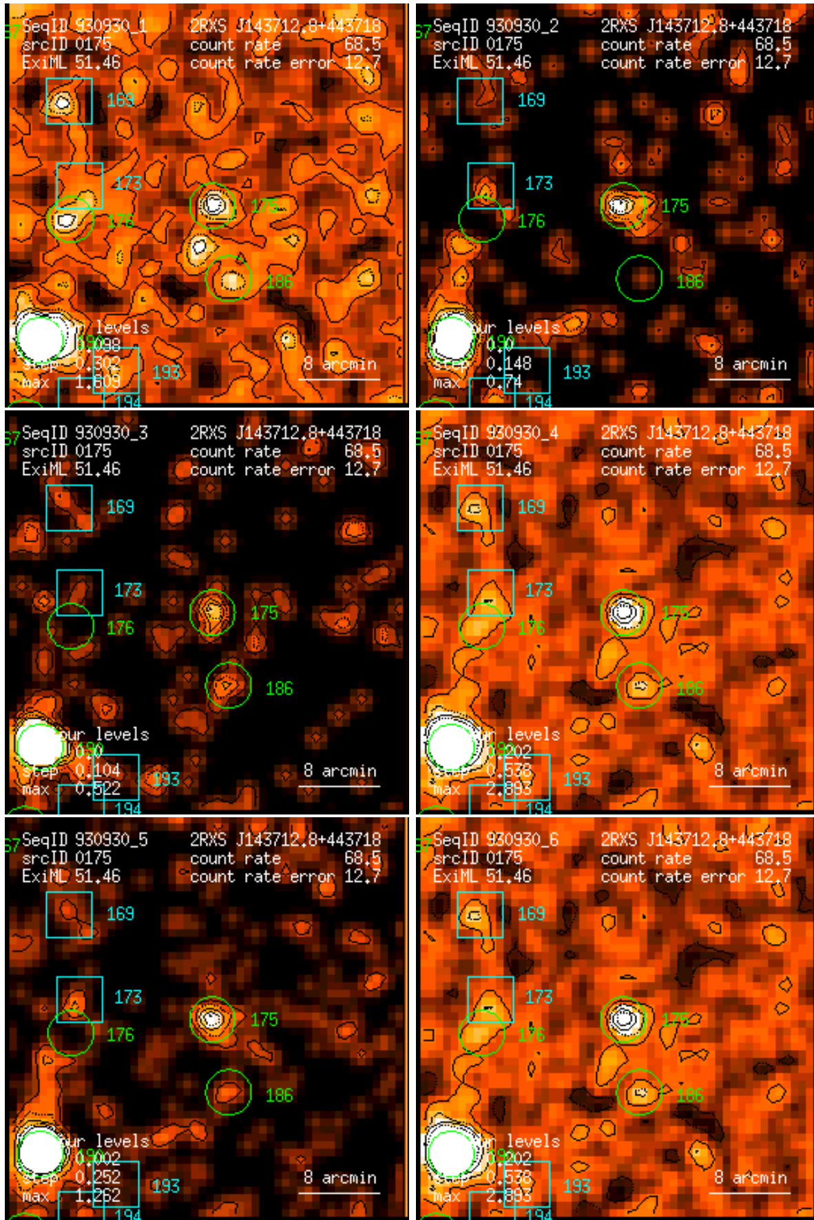
Figure 175: RASS 930930: detection 0175: band rate images, Gaussian filter: (1) PSPC channels 11 – 41, (2) 52 – 90, (3) 91 – 201, (4) 11 – 235, (5) 52 – 201, (6) 11 – 201. Broad band rates in counts/ks. Band rate contour levels in counts/ks/arcmin 2 .
