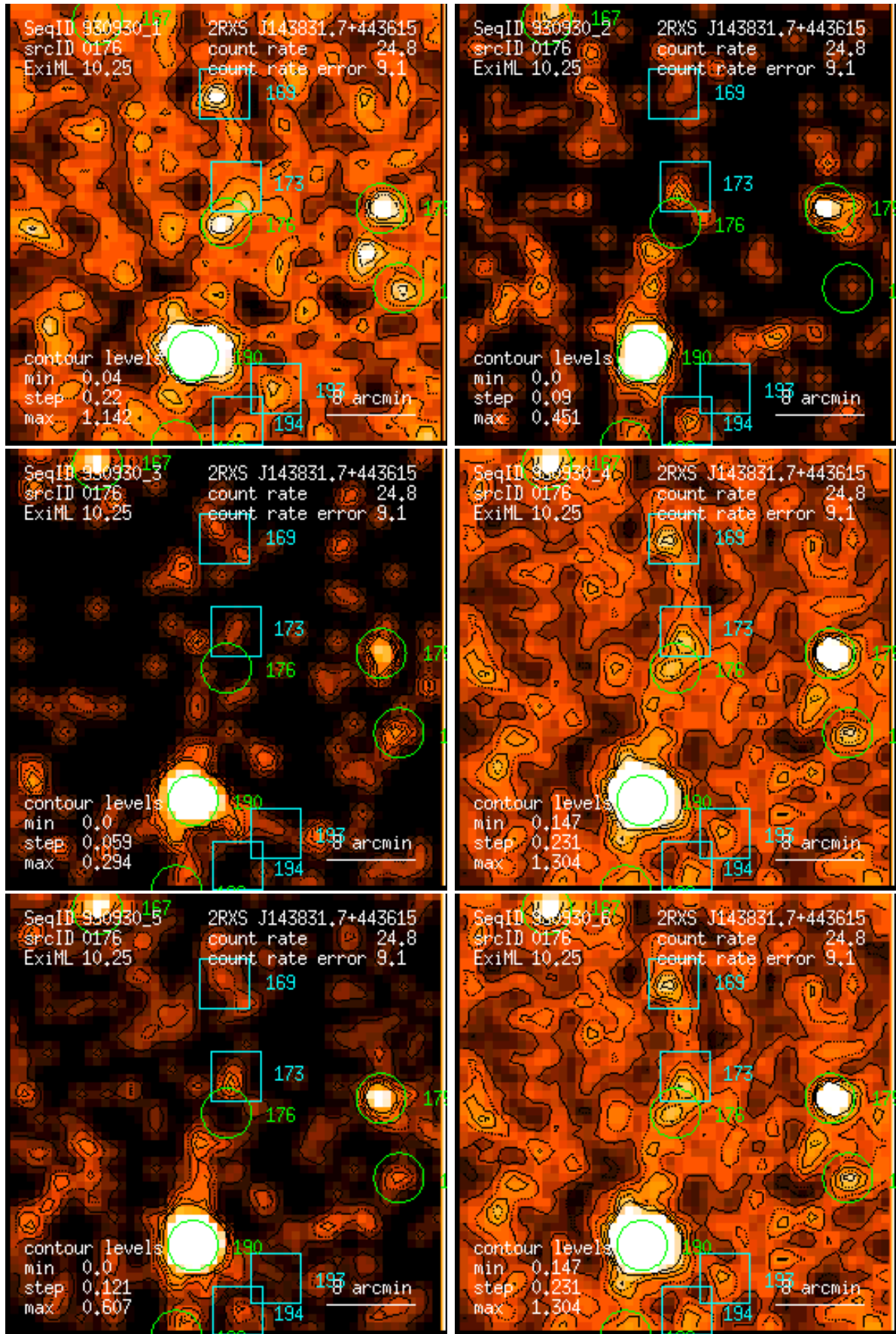
Figure 176: RASS 930930: detection 0176: band rate images, Gaussian filter: (1) PSPC channels 11 – 41, (2) 52 – 90, (3) 91 – 201, (4) 11 – 235, (5) 52 – 201, (6) 11 – 201. Broad band rates in counts/ks. Band rate contour levels in counts/ks/arcmin 2 .
