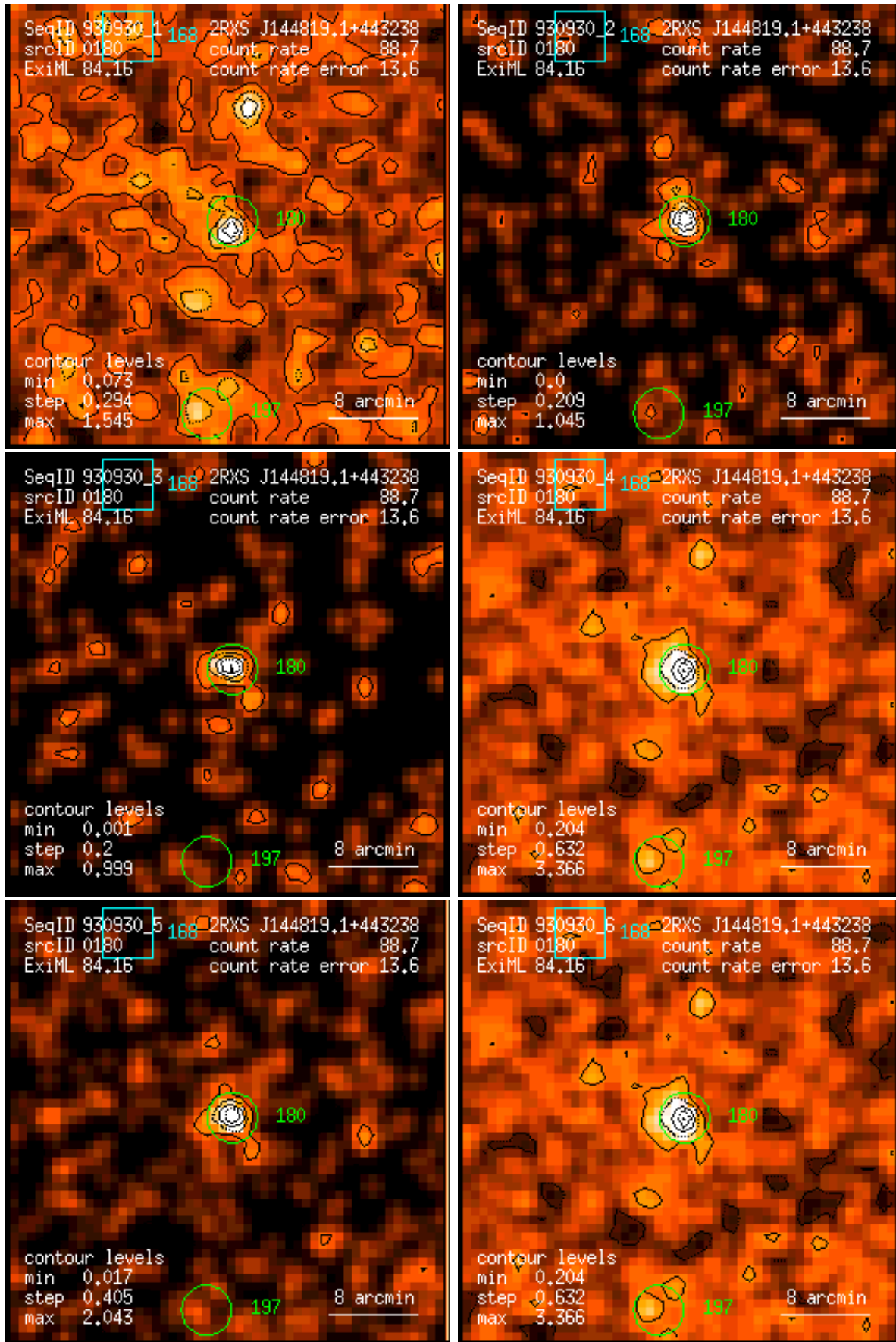
Figure 180: RASS 930930: detection 0180: band rate images, Gaussian filter: (1) PSPC channels 11 – 41, (2) 52 – 90, (3) 91 – 201, (4) 11 – 235, (5) 52 – 201, (6) 11 – 201. Broad band rates in counts/ks. Band rate contour levels in counts/ks/arcmin 2 .
