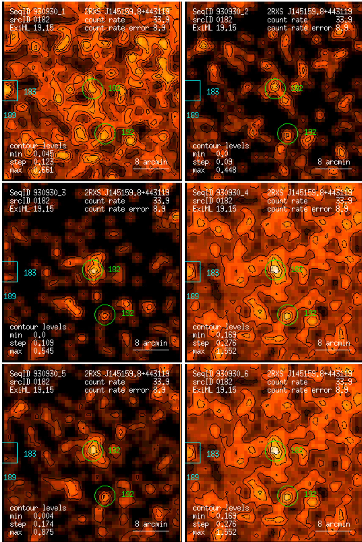
Figure 182: RASS 930930: detection 0182: band rate images, Gaussian filter: (1) PSPC channels 11 – 41, (2) 52 – 90, (3) 91 – 201, (4) 11 – 235, (5) 52 – 201, (6) 11 – 201. Broad band rates in counts/ks. Band rate contour levels in counts/ks/arcmin 2 .
