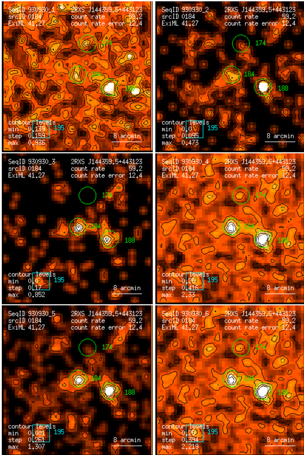
Figure 184: RASS 930930: detection 0184: band rate images, Gaussian filter: (1) PSPC channels 11 – 41, (2) 52 – 90, (3) 91 – 201, (4) 11 – 235, (5) 52 – 201, (6) 11 – 201. Broad band rates in counts/ks. Band rate contour levels in counts/ks/arcmin 2 .
