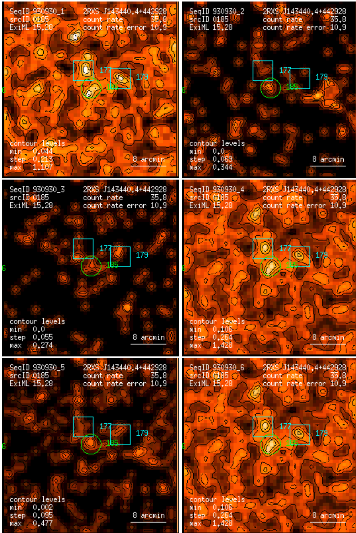
Figure 185: RASS 930930: detection 0185: band rate images, Gaussian filter: (1) PSPC channels 11 – 41, (2) 52 – 90, (3) 91 – 201, (4) 11 – 235, (5) 52 – 201, (6) 11 – 201. Broad band rates in counts/ks. Band rate contour levels in counts/ks/arcmin 2 .
