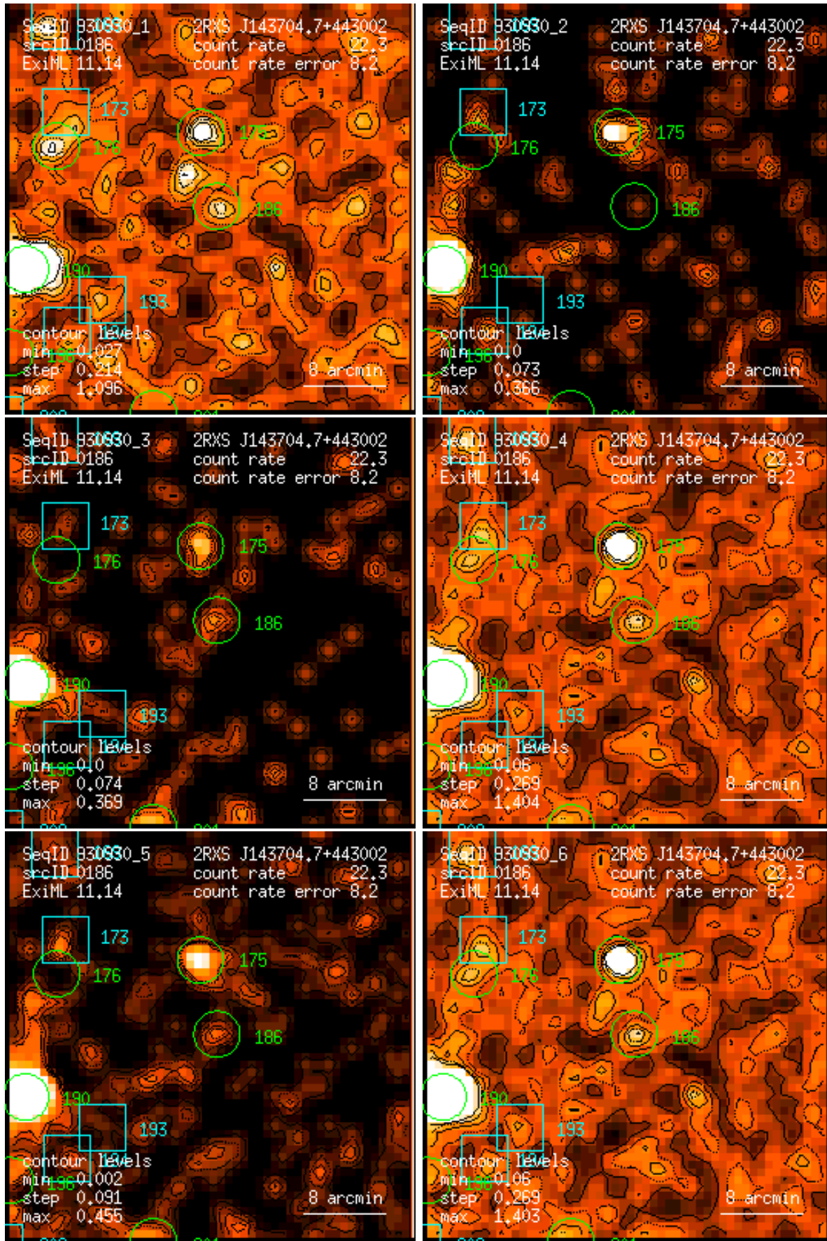
Figure 186: RASS 930930: detection 0186: band rate images, Gaussian filter: (1) PSPC channels 11 – 41, (2) 52 – 90, (3) 91 – 201, (4) 11 – 235, (5) 52 – 201, (6) 11 – 201. Broad band rates in counts/ks. Band rate contour levels in counts/ks/arcmin 2 .
