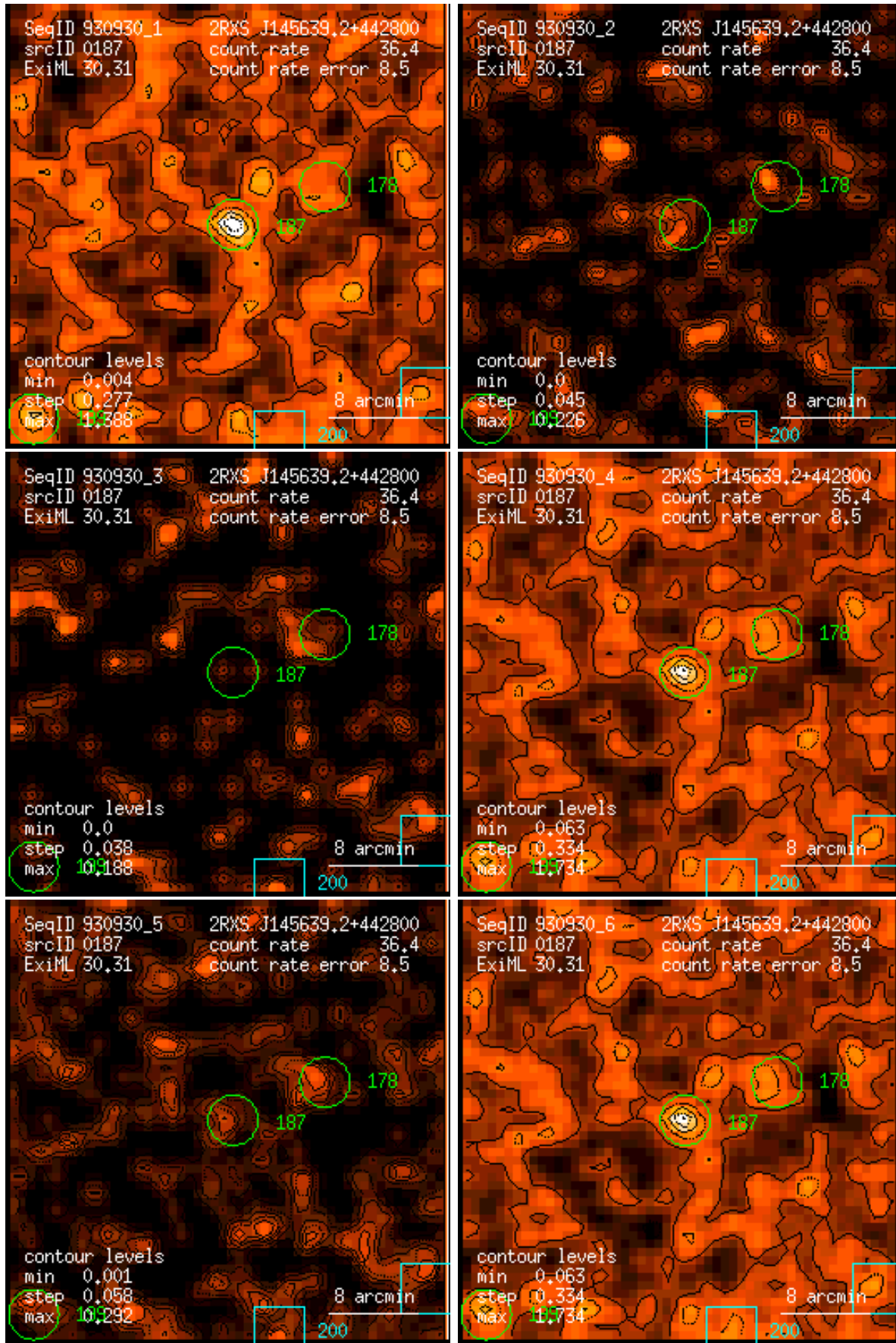
Figure 187: RASS 930930: detection 0187: band rate images, Gaussian filter: (1) PSPC channels 11 – 41, (2) 52 – 90, (3) 91 – 201, (4) 11 – 235, (5) 52 – 201, (6) 11 – 201. Broad band rates in counts/ks. Band rate contour levels in counts/ks/arcmin 2 .
