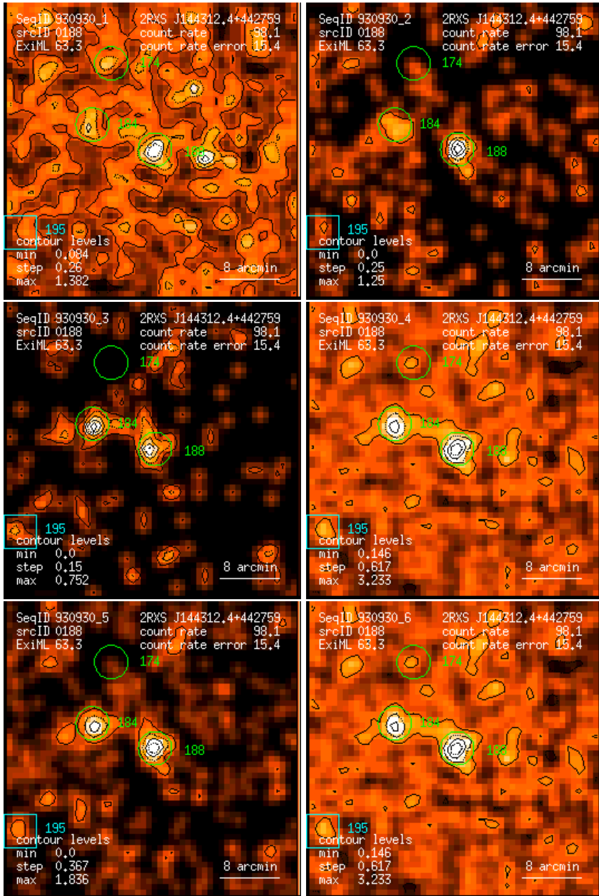
Figure 188: RASS 930930: detection 0188: band rate images, Gaussian filter: (1) PSPC channels 11 – 41, (2) 52 – 90, (3) 91 – 201, (4) 11 – 235, (5) 52 – 201, (6) 11 – 201. Broad band rates in counts/ks. Band rate contour levels in counts/ks/arcmin 2 .
