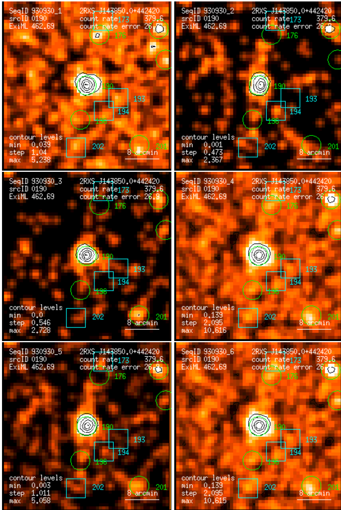
Figure 190: RASS 930930: detection 0190: band rate images, Gaussian filter: (1) PSPC channels 11 – 41, (2) 52 – 90, (3) 91 – 201, (4) 11 – 235, (5) 52 – 201, (6) 11 – 201. Broad band rates in counts/ks. Band rate contour levels in counts/ks/arcmin 2 .
