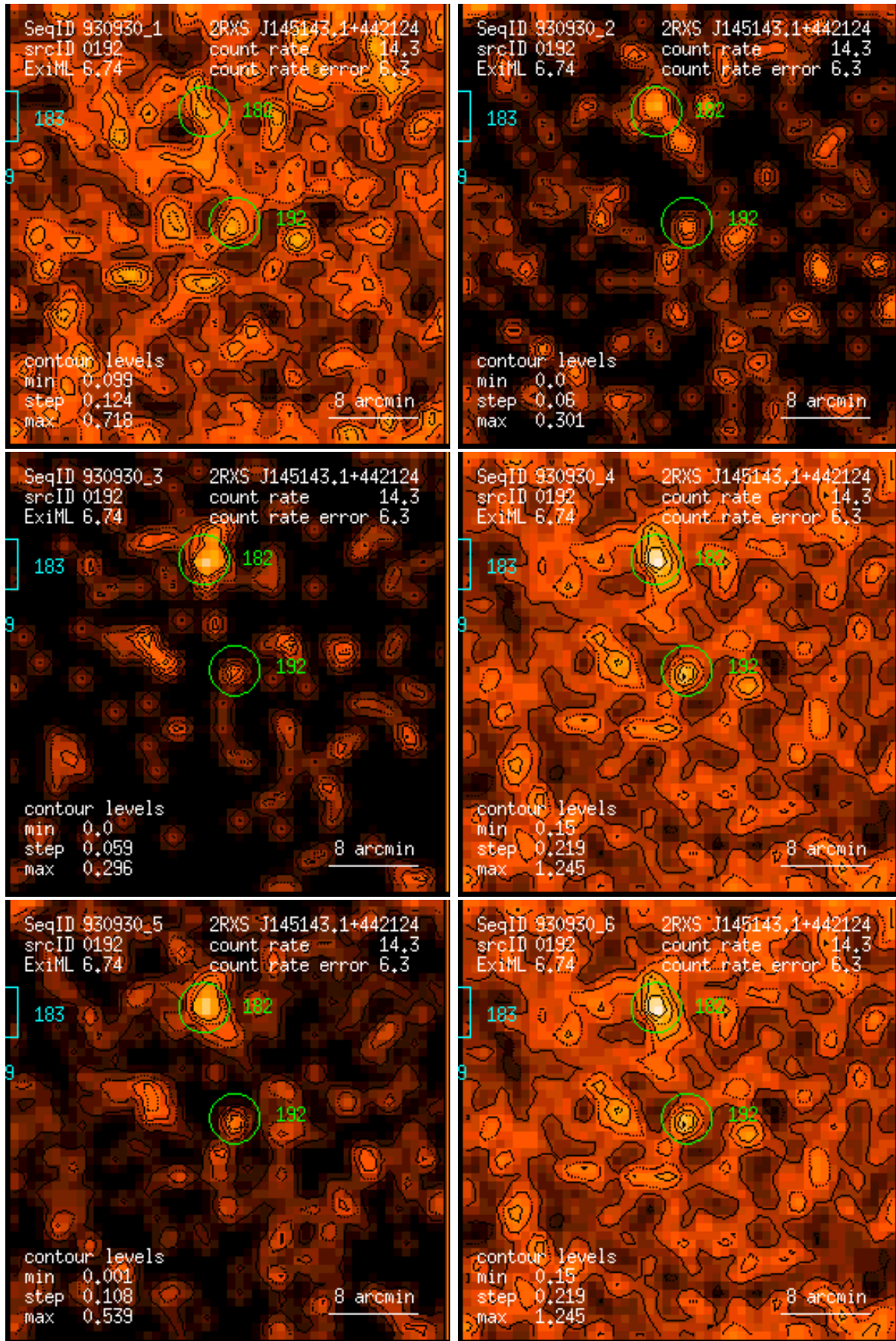
Figure 192: RASS 930930: detection 0192: band rate images, Gaussian filter: (1) PSPC channels 11 – 41, (2) 52 – 90, (3) 91 – 201, (4) 11 – 235, (5) 52 – 201, (6) 11 – 201. Broad band rates in counts/ks. Band rate contour levels in counts/ks/arcmin 2 .
