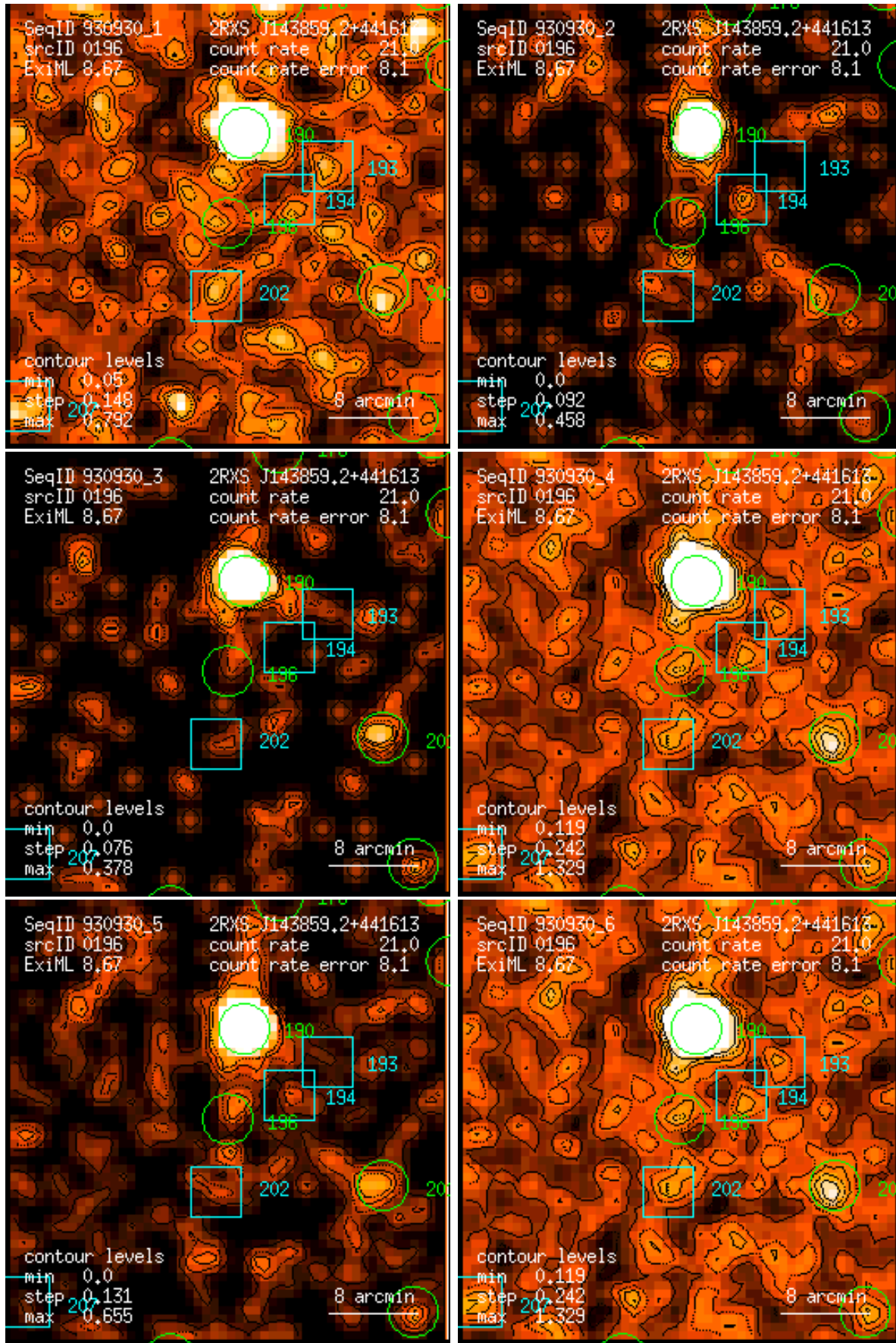
Figure 196: RASS 930930: detection 0196: band rate images, Gaussian filter: (1) PSPC channels 11 – 41, (2) 52 – 90, (3) 91 – 201, (4) 11 – 235, (5) 52 – 201, (6) 11 – 201. Broad band rates in counts/ks. Band rate contour levels in counts/ks/arcmin 2 .
