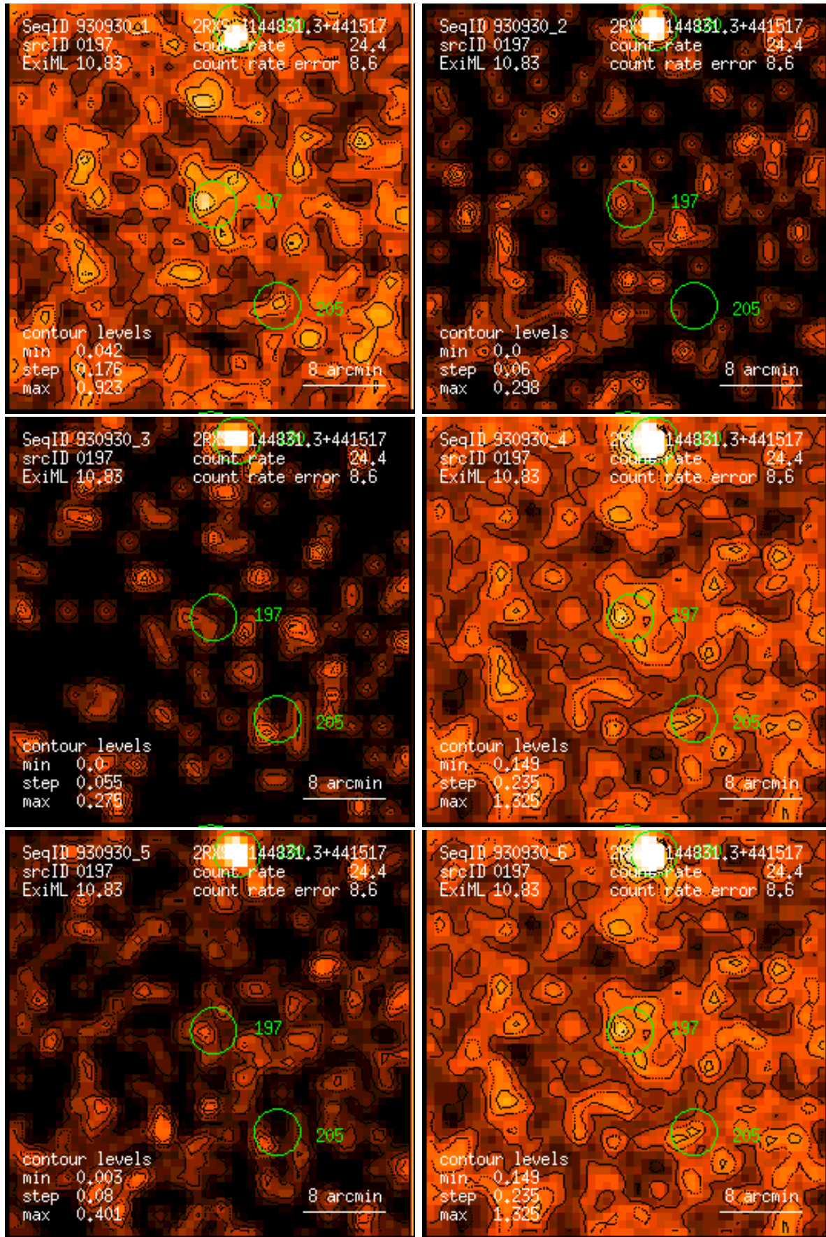
Figure 197: RASS 930930: detection 0197: band rate images, Gaussian filter: (1) PSPC channels 11 – 41, (2) 52 – 90, (3) 91 – 201, (4) 11 – 235, (5) 52 – 201, (6) 11 – 201. Broad band rates in counts/ks. Band rate contour levels in counts/ks/arcmin 2 .
