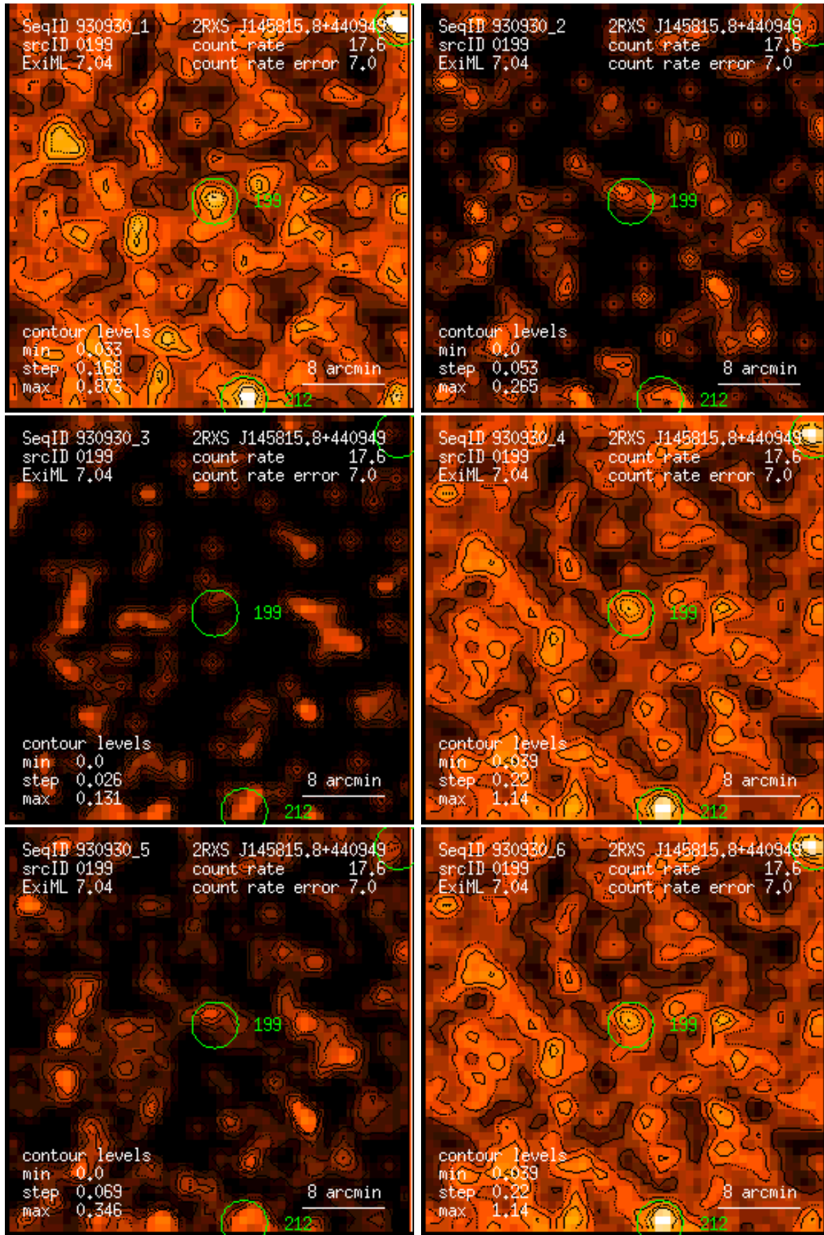
Figure 199: RASS 930930: detection 0199: band rate images, Gaussian filter: (1) PSPC channels 11 – 41, (2) 52 – 90, (3) 91 – 201, (4) 11 – 235, (5) 52 – 201, (6) 11 – 201. Broad band rates in counts/ks. Band rate contour levels in counts/ks/arcmin 2 .
