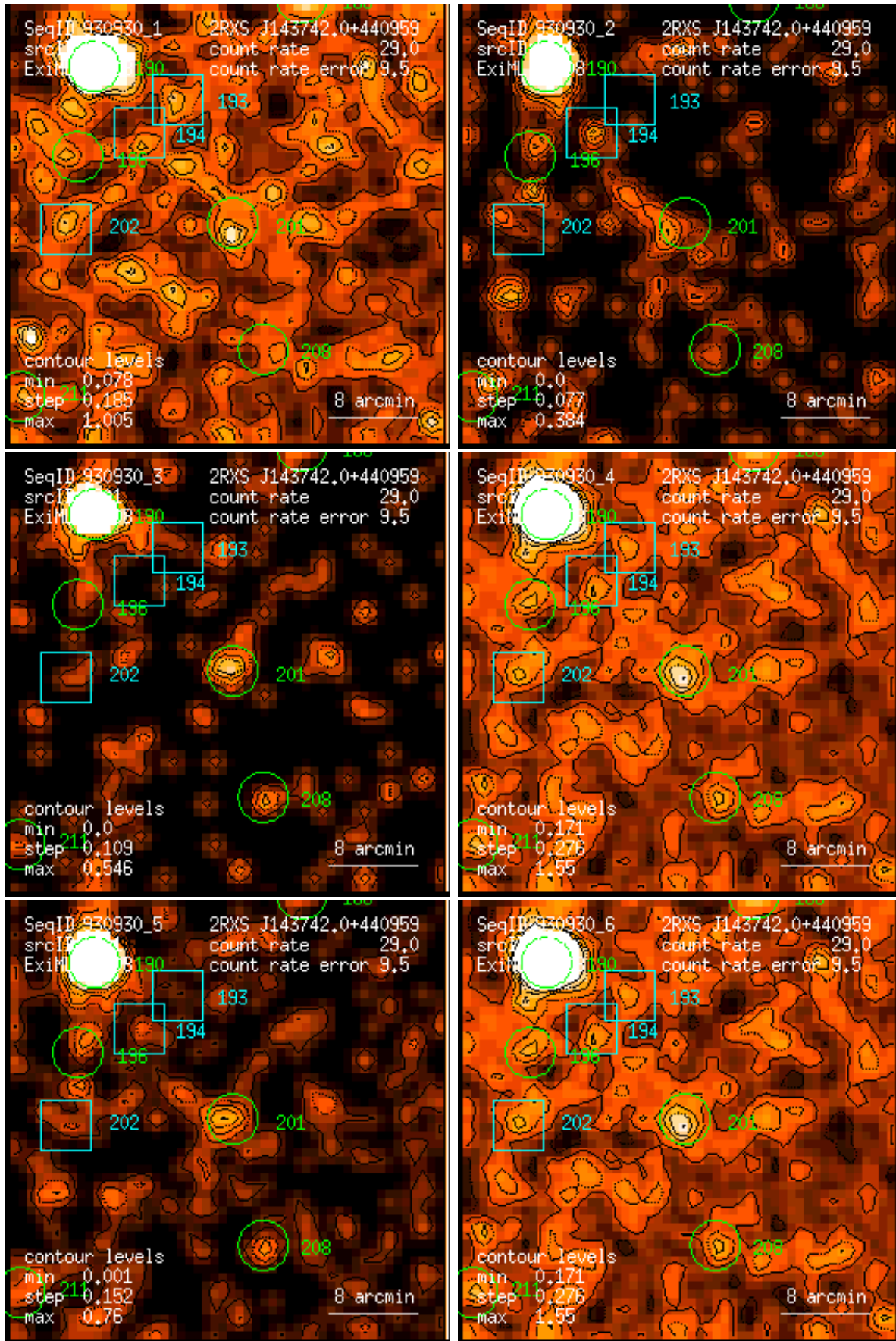
Figure 201: RASS 930930: detection 0201: band rate images, Gaussian filter: (1) PSPC channels 11 – 41, (2) 52 – 90, (3) 91 – 201, (4) 11 – 235, (5) 52 – 201, (6) 11 – 201. Broad band rates in counts/ks. Band rate contour levels in counts/ks/arcmin 2 .
