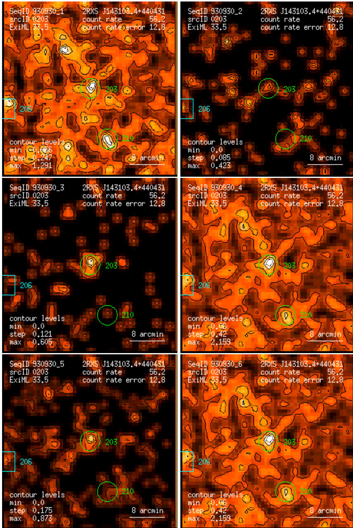
Figure 203: RASS 930930: detection 0203: band rate images, Gaussian filter: (1) PSPC channels 11 – 41, (2) 52 – 90, (3) 91 – 201, (4) 11 – 235, (5) 52 – 201, (6) 11 – 201. Broad band rates in counts/ks. Band rate contour levels in counts/ks/arcmin 2 .
