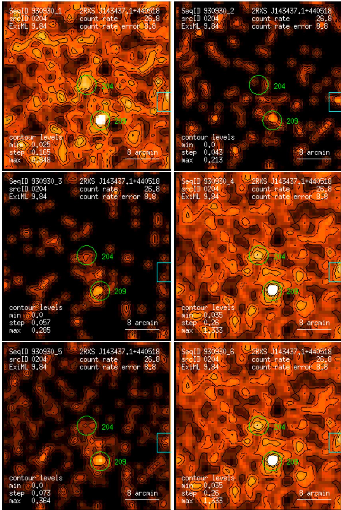
Figure 204: RASS 930930: detection 0204: band rate images, Gaussian filter: (1) PSPC channels 11 – 41, (2) 52 – 90, (3) 91 – 201, (4) 11 – 235, (5) 52 – 201, (6) 11 – 201. Broad band rates in counts/ks. Band rate contour levels in counts/ks/arcmin 2 .
