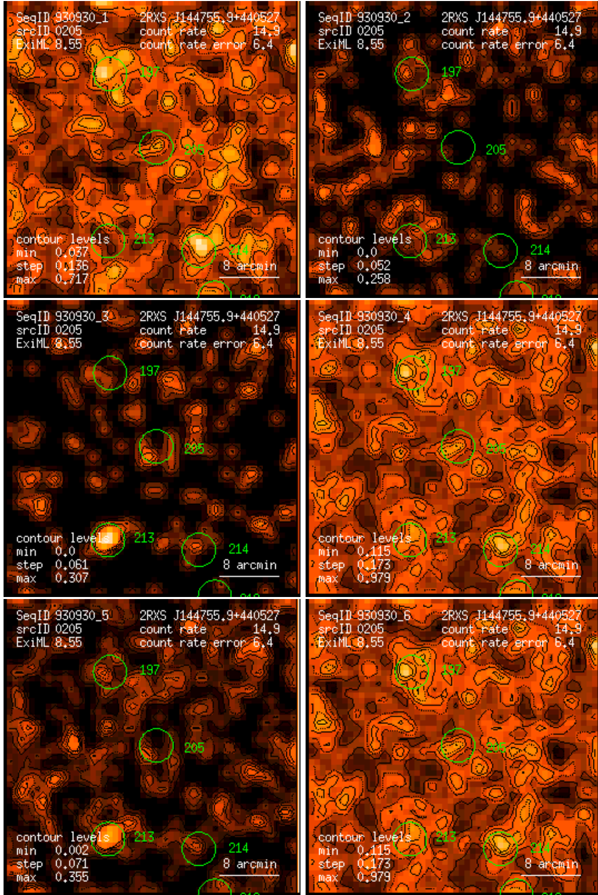
Figure 205: RASS 930930: detection 0205: band rate images, Gaussian filter: (1) PSPC channels 11 – 41, (2) 52 – 90, (3) 91 – 201, (4) 11 – 235, (5) 52 – 201, (6) 11 – 201. Broad band rates in counts/ks. Band rate contour levels in counts/ks/arcmin 2 .
