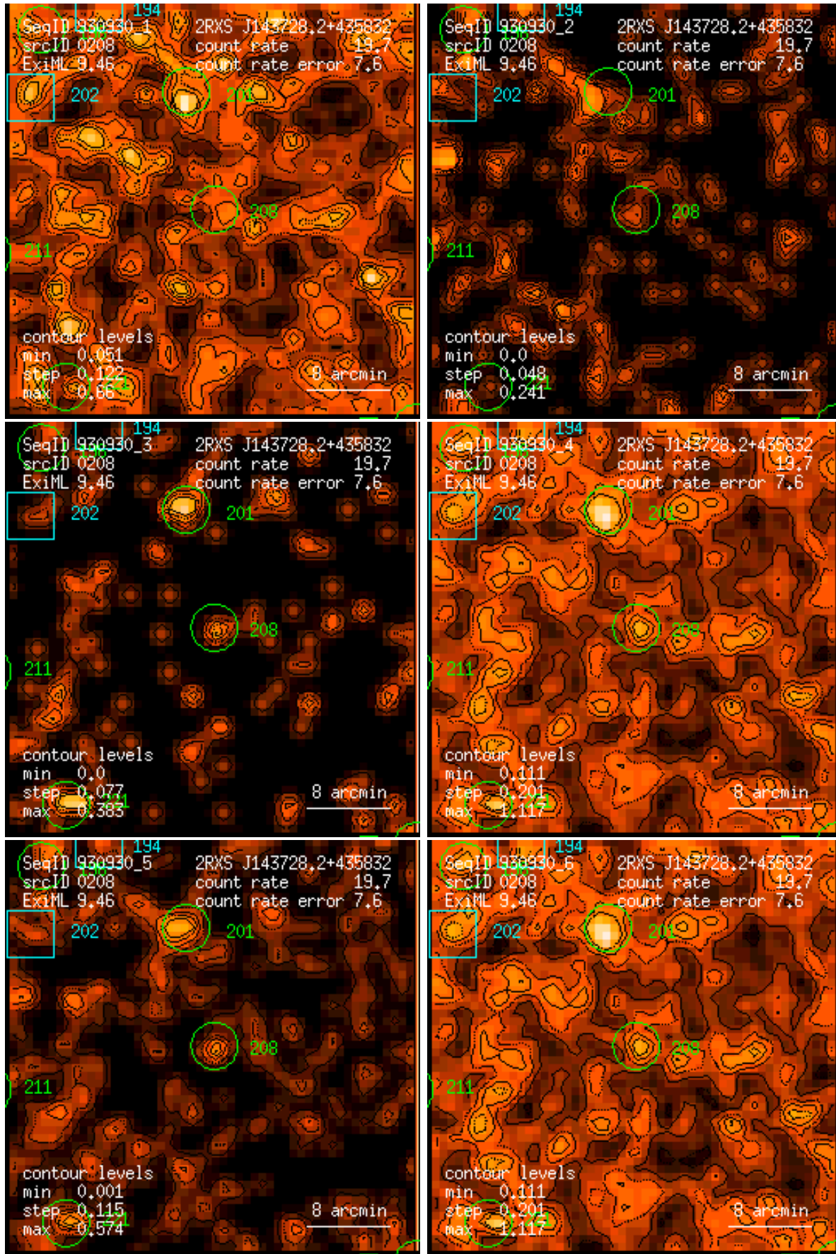
Figure 208: RASS 930930: detection 0208: band rate images, Gaussian filter: (1) PSPC channels 11 – 41, (2) 52 – 90, (3) 91 – 201, (4) 11 – 235, (5) 52 – 201, (6) 11 – 201. Broad band rates in counts/ks. Band rate contour levels in counts/ks/arcmin 2 .
