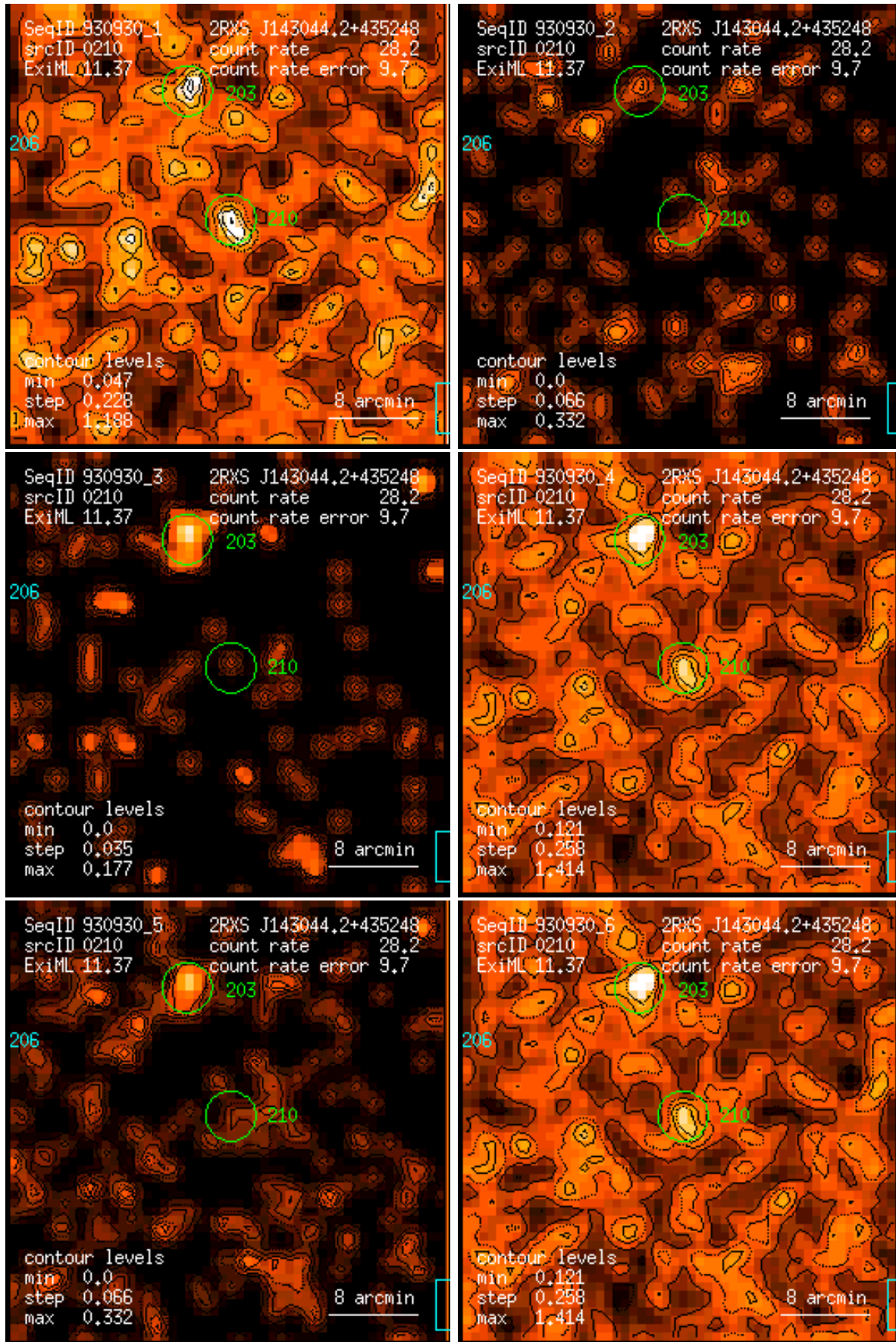
Figure 210: RASS 930930: detection 0210: band rate images, Gaussian filter: (1) PSPC channels 11 – 41, (2) 52 – 90, (3) 91 – 201, (4) 11 – 235, (5) 52 – 201, (6) 11 – 201. Broad band rates in counts/ks. Band rate contour levels in counts/ks/arcmin 2 .
