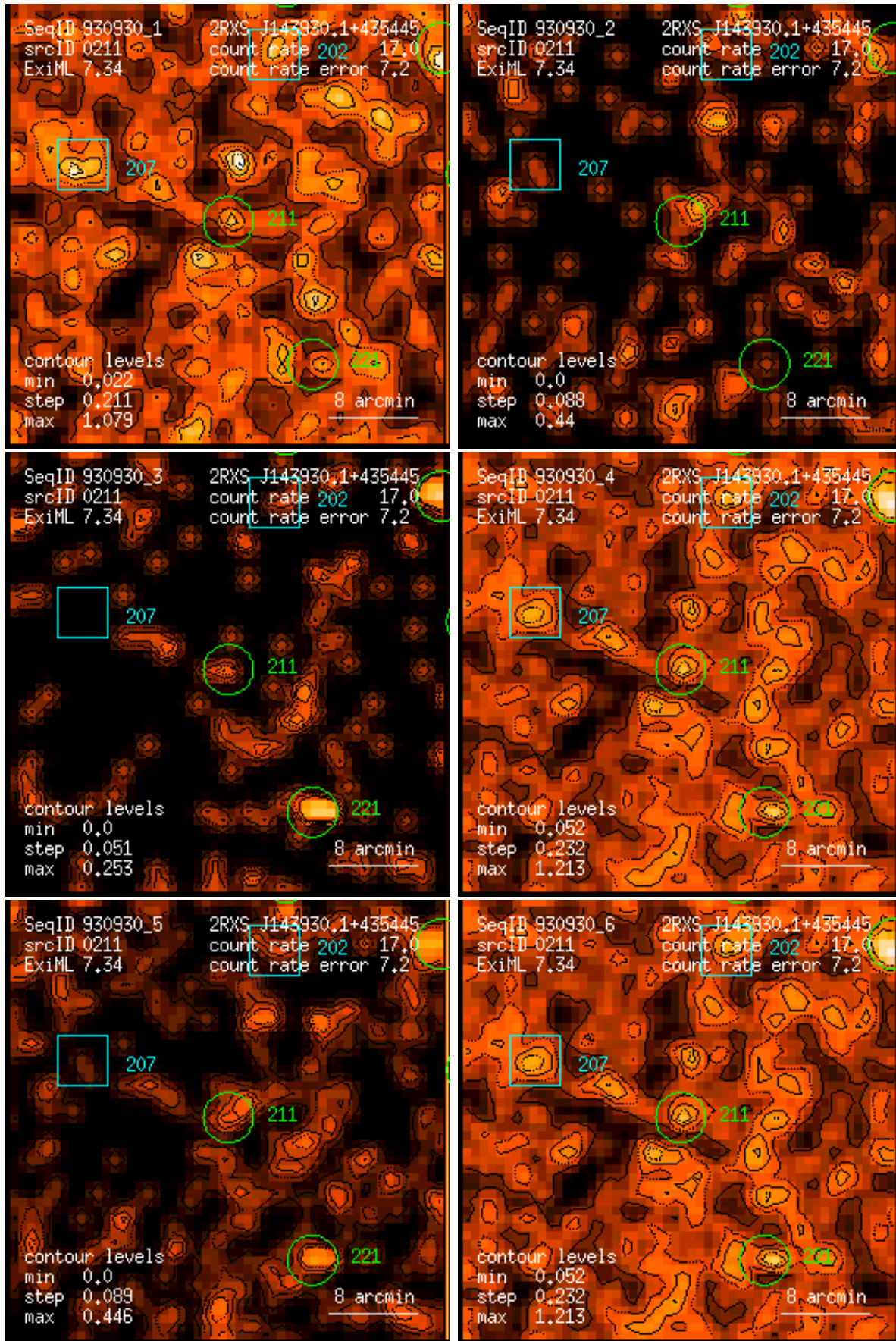
Figure 211: RASS 930930: detection 0211: band rate images, Gaussian filter: (1) PSPC channels 11 – 41, (2) 52 – 90, (3) 91 – 201, (4) 11 – 235, (5) 52 – 201, (6) 11 – 201. Broad band rates in counts/ks. Band rate contour levels in counts/ks/arcmin 2 .
