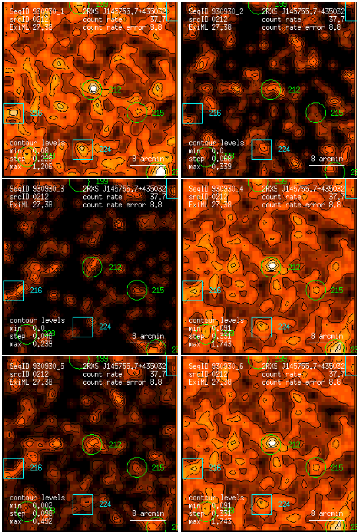
Figure 212: RASS 930930: detection 0212: band rate images, Gaussian filter: (1) PSPC channels 11 – 41, (2) 52 – 90, (3) 91 – 201, (4) 11 – 235, (5) 52 – 201, (6) 11 – 201. Broad band rates in counts/ks. Band rate contour levels in counts/ks/arcmin 2 .
