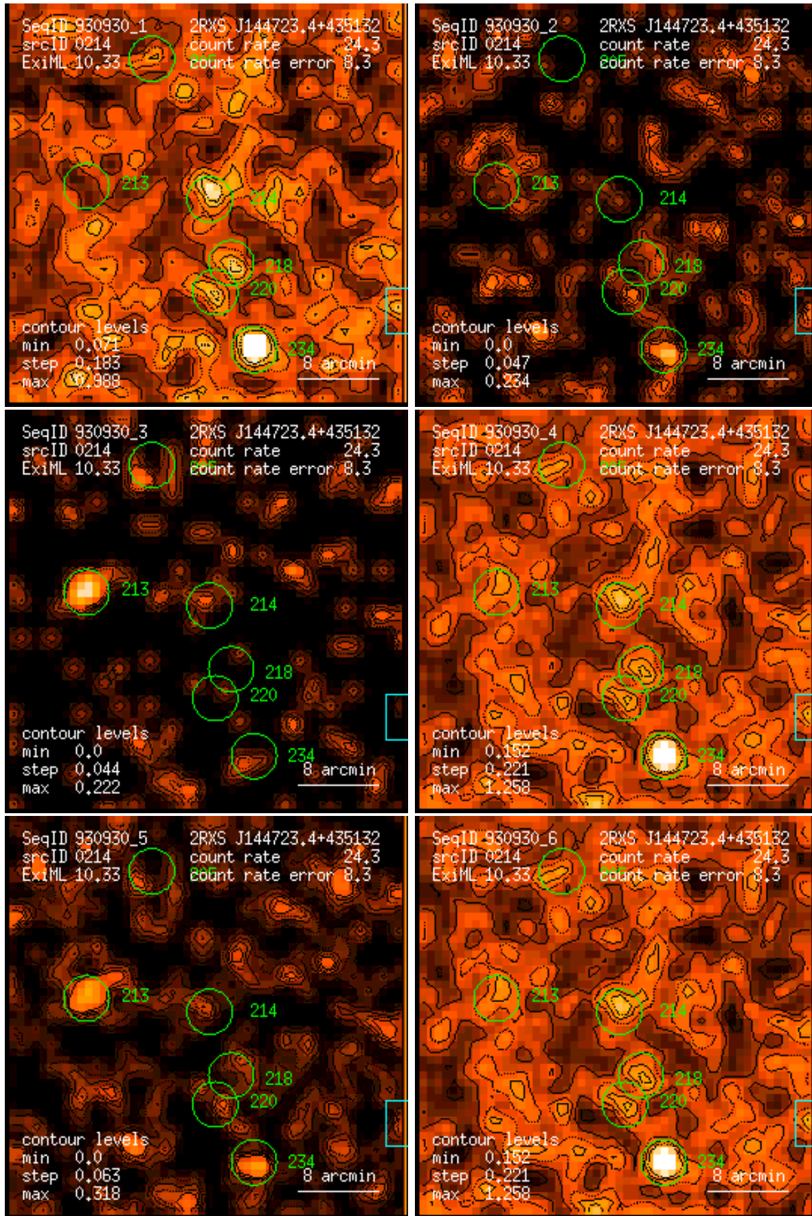
Figure 214: RASS 930930: detection 0214: band rate images, Gaussian filter: (1) PSPC channels 11 – 41, (2) 52 – 90, (3) 91 – 201, (4) 11 – 235, (5) 52 – 201, (6) 11 – 201. Broad band rates in counts/ks. Band rate contour levels in counts/ks/arcmin 2 .
