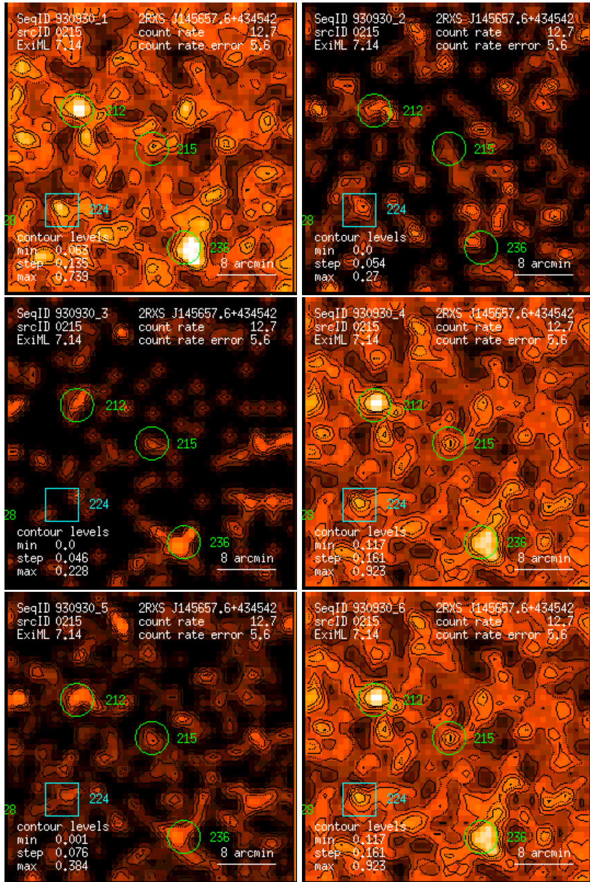
Figure 215: RASS 930930: detection 0215: band rate images, Gaussian filter: (1) PSPC channels 11 – 41, (2) 52 – 90, (3) 91 – 201, (4) 11 – 235, (5) 52 – 201, (6) 11 – 201. Broad band rates in counts/ks. Band rate contour levels in counts/ks/arcmin 2 .
