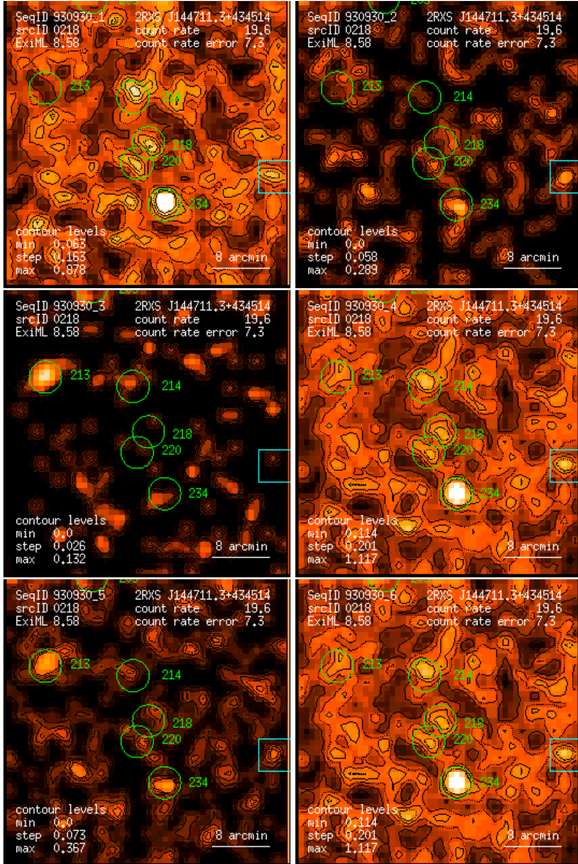
Figure 218: RASS 930930: detection 0218: band rate images, Gaussian filter: (1) PSPC channels 11 – 41, (2) 52 – 90, (3) 91 – 201, (4) 11 – 235, (5) 52 – 201, (6) 11 – 201. Broad band rates in counts/ks. Band rate contour levels in counts/ks/arcmin 2 .
