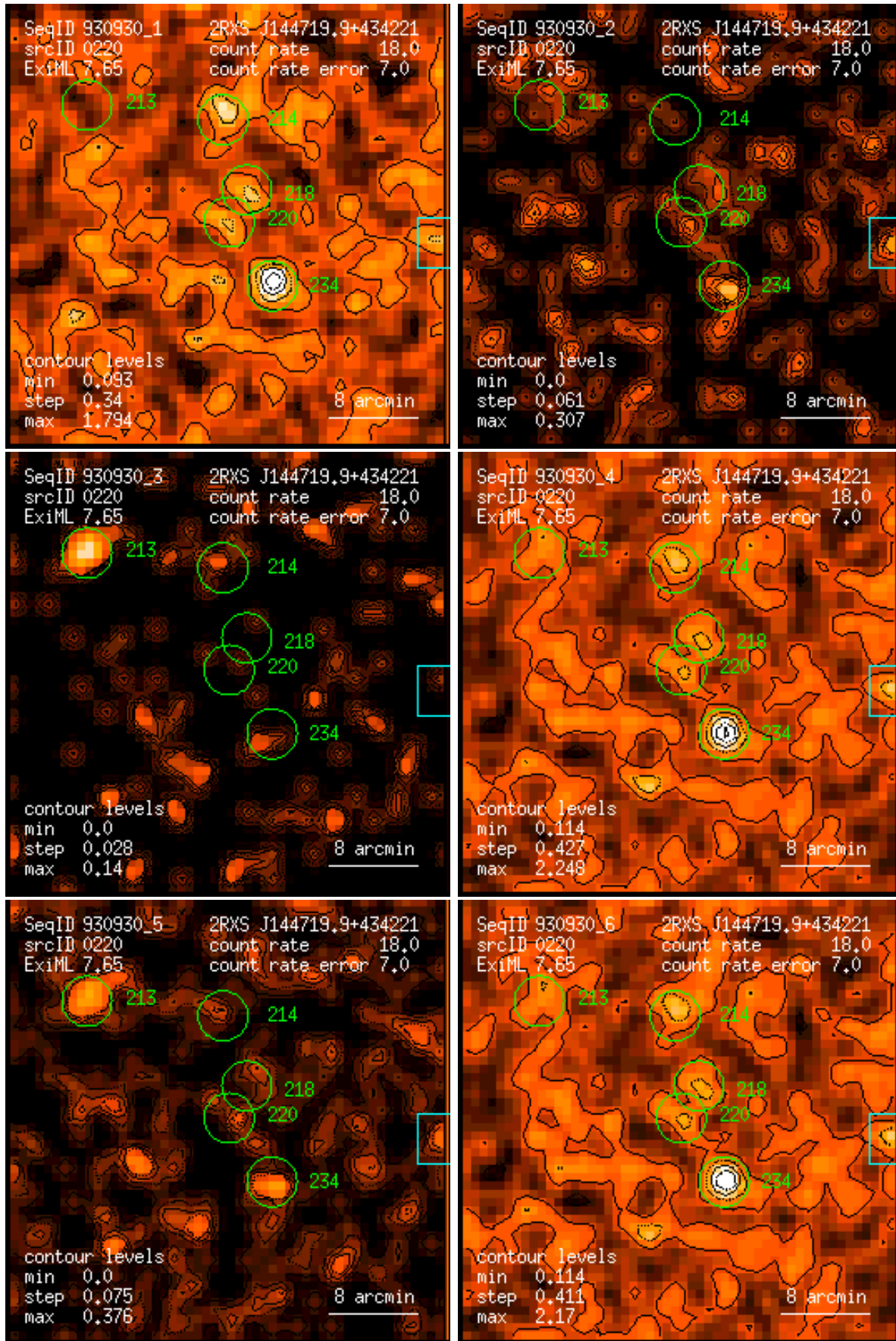
Figure 220: RASS 930930: detection 0220: band rate images, Gaussian filter: (1) PSPC channels 11 – 41, (2) 52 – 90, (3) 91 – 201, (4) 11 – 235, (5) 52 – 201, (6) 11 – 201. Broad band rates in counts/ks. Band rate contour levels in counts/ks/arcmin 2 .
