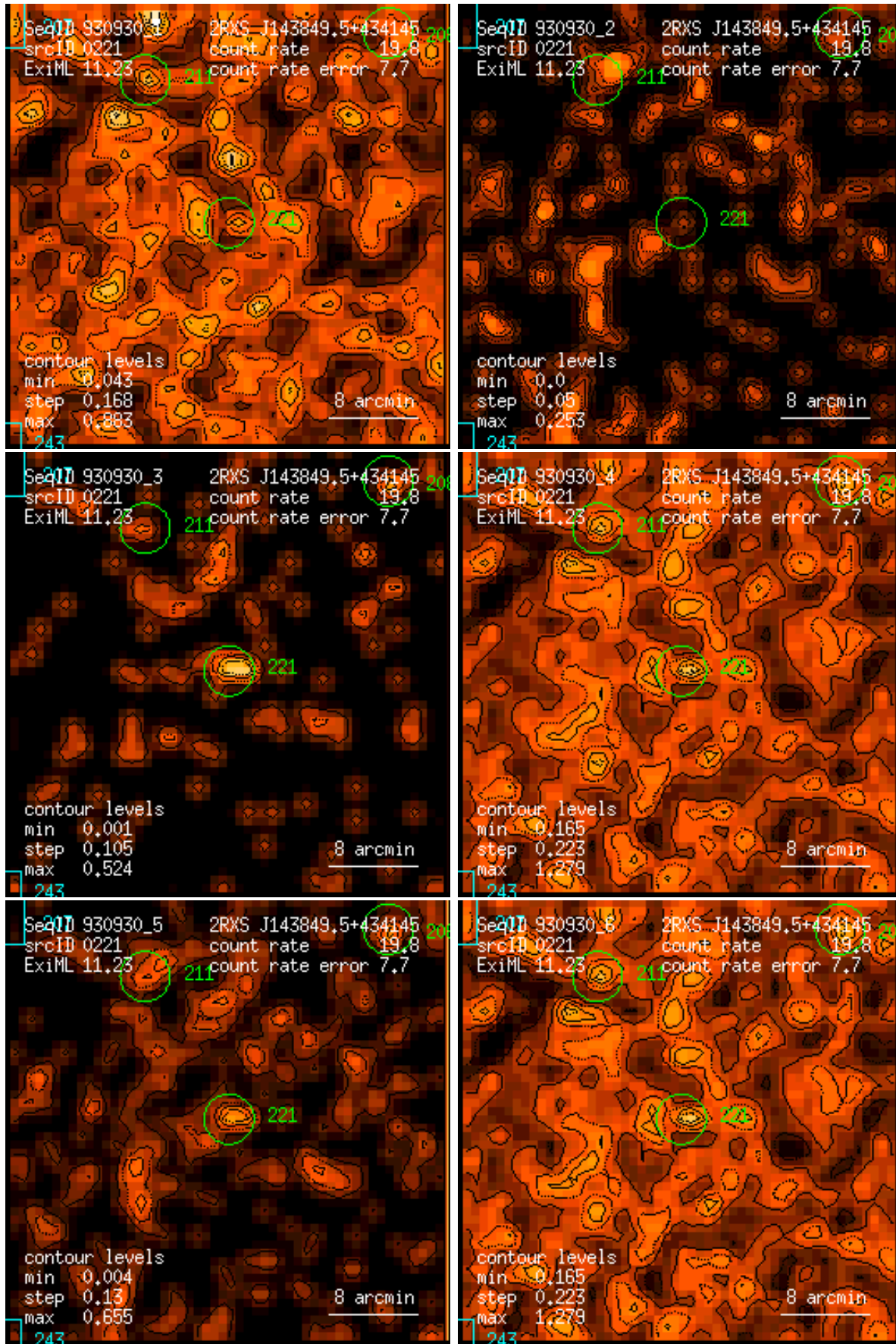
Figure 221: RASS 930930: detection 0221: band rate images, Gaussian filter: (1) PSPC channels 11 – 41, (2) 52 – 90, (3) 91 – 201, (4) 11 – 235, (5) 52 – 201, (6) 11 – 201. Broad band rates in counts/ks. Band rate contour levels in counts/ks/arcmin 2 .
