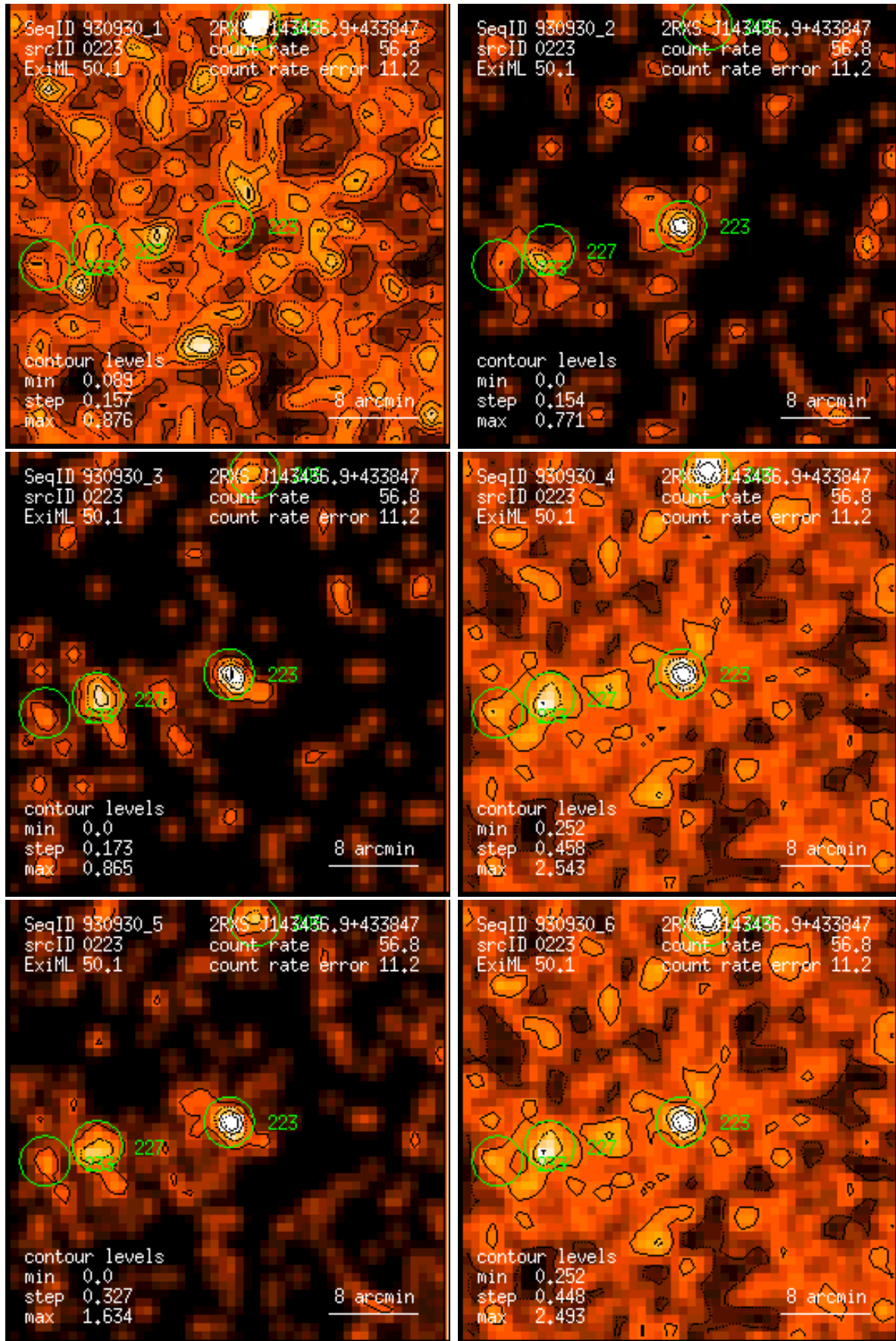
Figure 223: RASS 930930: detection 0223: band rate images, Gaussian filter: (1) PSPC channels 11 – 41, (2) 52 – 90, (3) 91 – 201, (4) 11 – 235, (5) 52 – 201, (6) 11 – 201. Broad band rates in counts/ks. Band rate contour levels in counts/ks/arcmin 2 .
