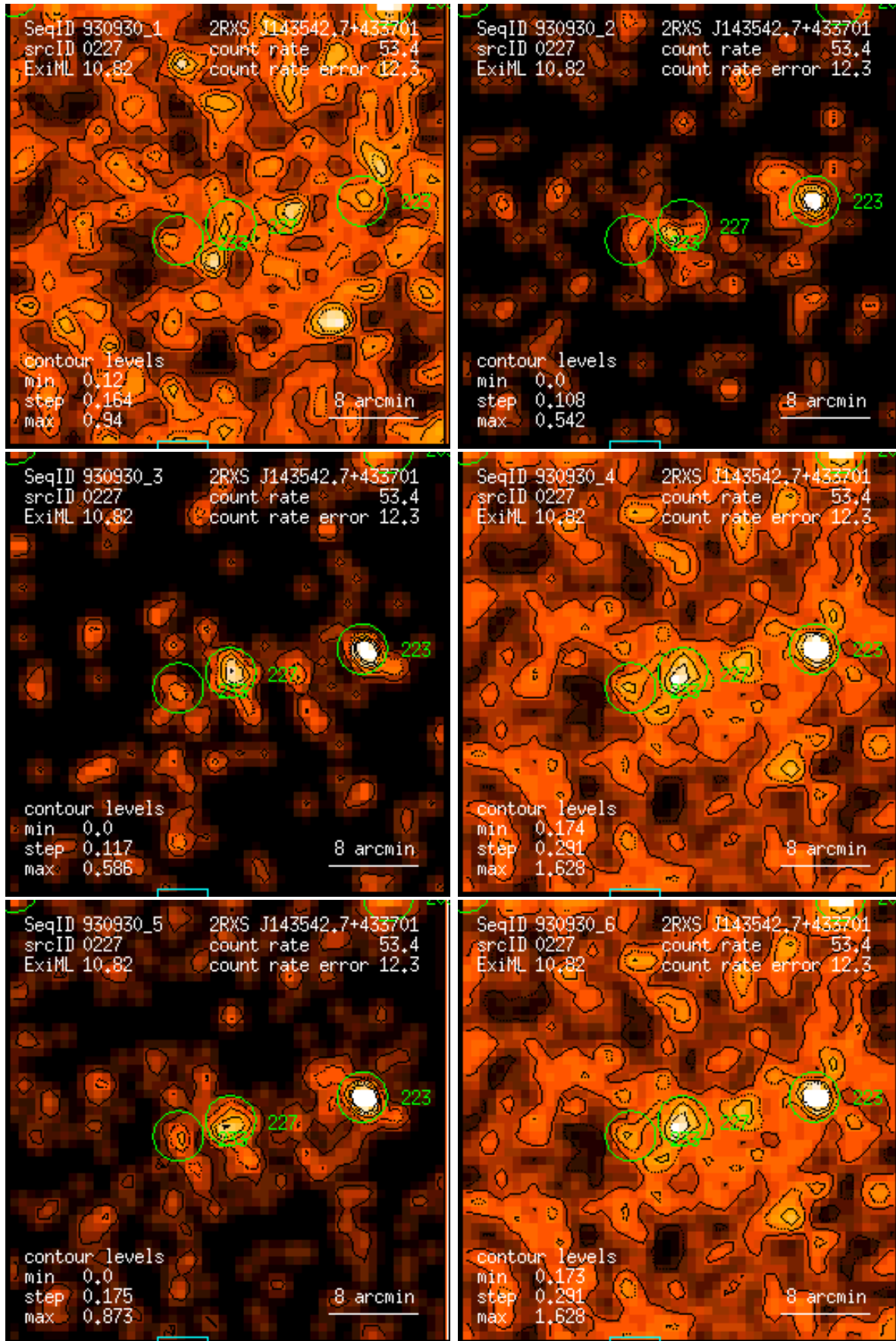
Figure 227: RASS 930930: detection 0227: band rate images, Gaussian filter: (1) PSPC channels 11 – 41, (2) 52 – 90, (3) 91 – 201, (4) 11 – 235, (5) 52 – 201, (6) 11 – 201. Broad band rates in counts/ks. Band rate contour levels in counts/ks/arcmin 2 .
