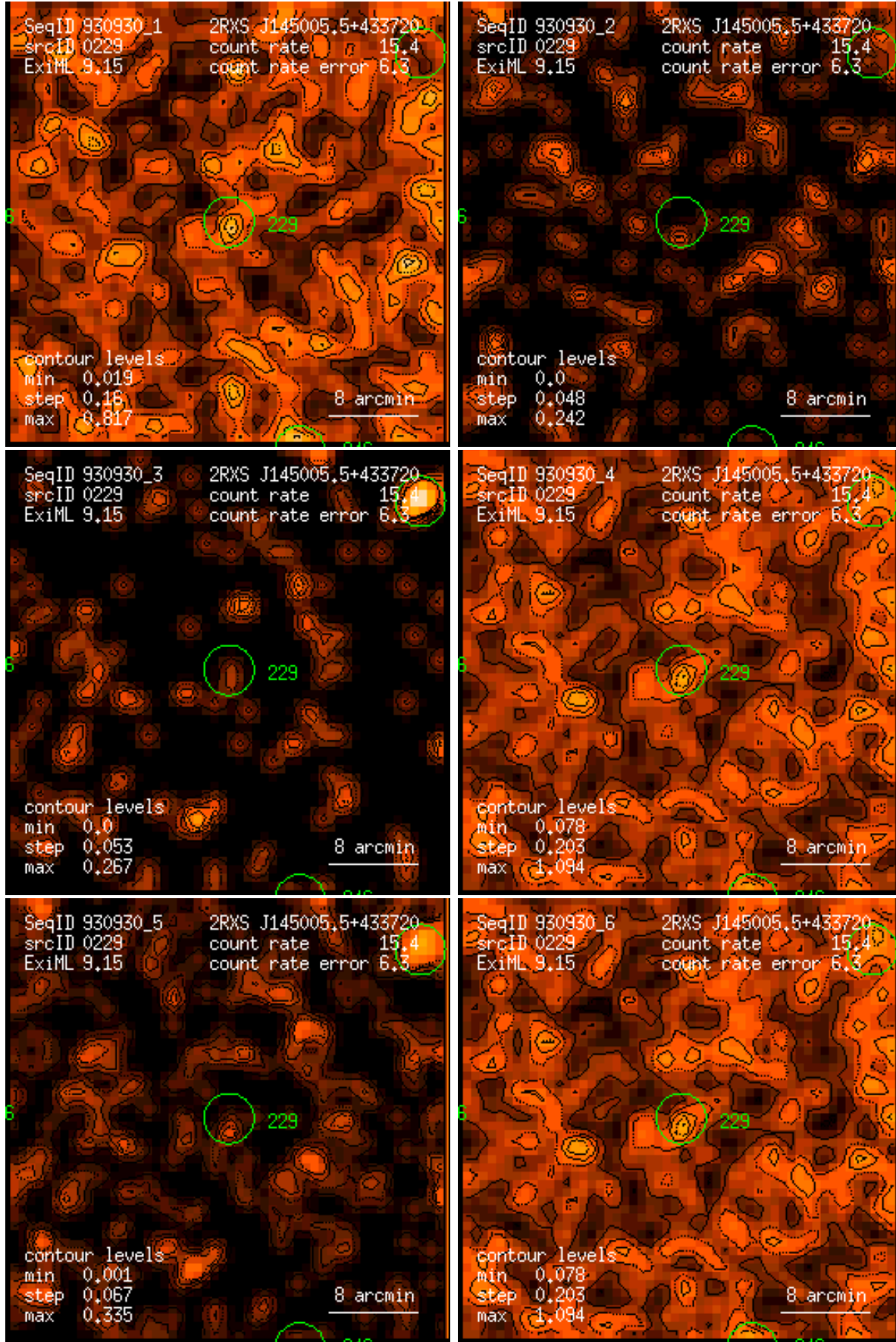
Figure 229: RASS 930930: detection 0229: band rate images, Gaussian filter: (1) PSPC channels 11 – 41, (2) 52 – 90, (3) 91 – 201, (4) 11 – 235, (5) 52 – 201, (6) 11 – 201. Broad band rates in counts/ks. Band rate contour levels in counts/ks/arcmin 2 .
