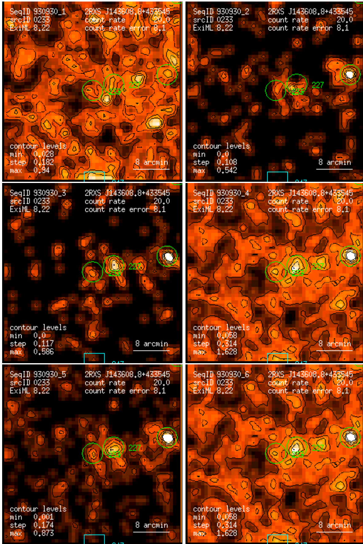
Figure 233: RASS 930930: detection 0233: band rate images, Gaussian filter: (1) PSPC channels 11 – 41, (2) 52 – 90, (3) 91 – 201, (4) 11 – 235, (5) 52 – 201, (6) 11 – 201. Broad band rates in counts/ks. Band rate contour levels in counts/ks/arcmin 2 .
