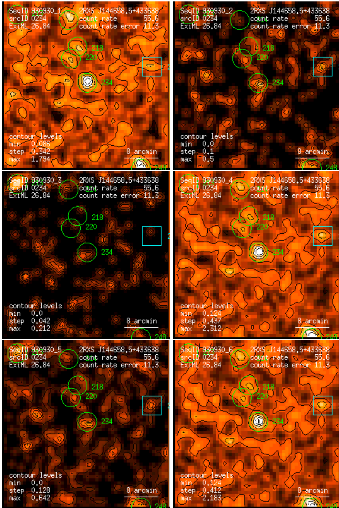
Figure 234: RASS 930930: detection 0234: band rate images, Gaussian filter: (1) PSPC channels 11 – 41, (2) 52 – 90, (3) 91 – 201, (4) 11 – 235, (5) 52 – 201, (6) 11 – 201. Broad band rates in counts/ks. Band rate contour levels in counts/ks/arcmin 2 .
